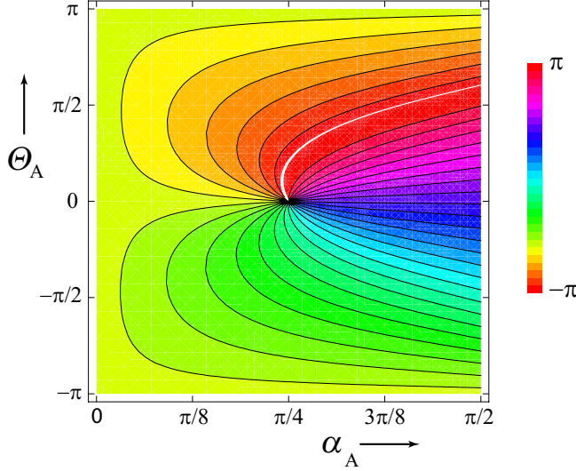
Figure 5.6: Color-coded plot of the phase of the final state E as a function of the initial state A as described by the two parameters \alpha_A and \theta_A [cf. Eq. (5.1)]. In this example \phi_1 = 3\pi/4 , and \phi_2 = 1.8 .
