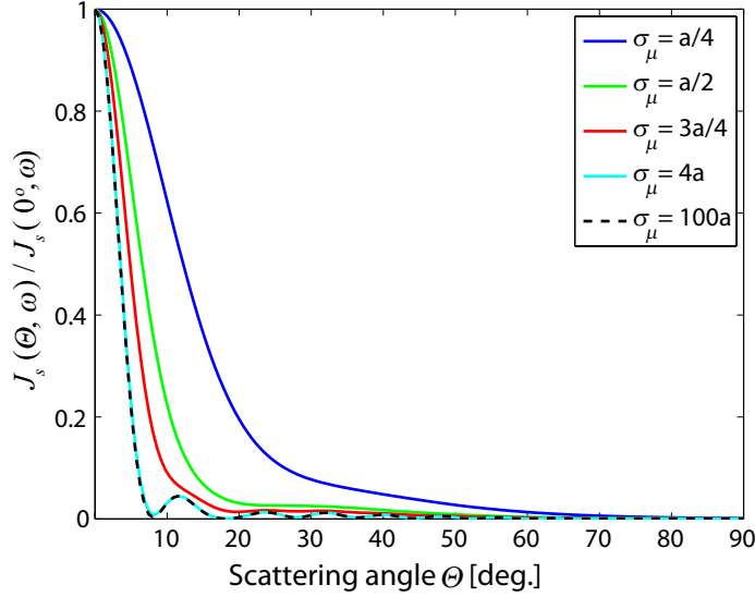
Figure 7.2: (Color on-line) The angular distribution of the normalized radiant intensity J_s(\theta, \omega)/J_s(0^\circ, \omega) of the scattered field for selected values of the transverse spectral coherence length \sigma_\mu of the incident beam, with the choices a = 4\lambda and n = 1.5 .
