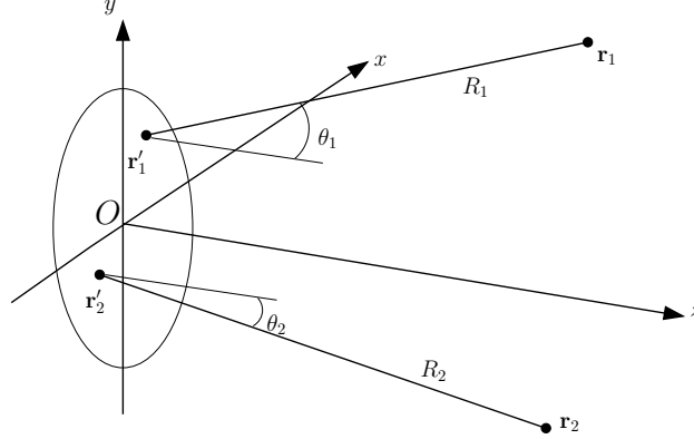
Figure 1.2: Illustrating the notation for propagation of the cross-spectral density from the source plane into the half space z > 0 .
