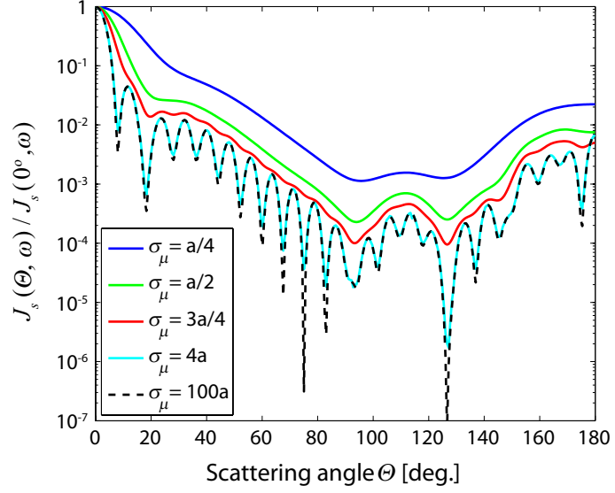
Figure 7.3: (Color on-line) The normalized radiant intensity J(\theta, \omega)/J_s(0^\circ, \omega) of the scattered field for selected values of the transverse spectral coherence length \sigma_\mu , plotted on a logarithmic scale. The sphere radius a has been taken to be 4\lambda , and the refractive index n = 1.5 .
