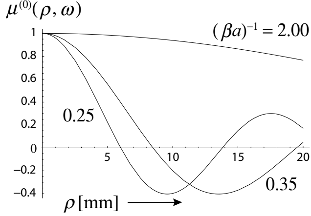
Figure 2.5: The spectral degree of coherence of the field in the aperture \mu^{(0)}(\rho, \omega) for three different values of (\beta a)^{-1} , as discussed in the text. In this example \lambda = 500 nm, a = 0.01 m, and f = 2 m.
