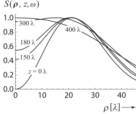
Figure 3.3: The normalized spectral density S(\boldsymbol{\rho}, z, \omega) , calculated from Eq. (3.18), in several cross-sections of the beam. In this example \sigma_S = 15\lambda and \sigma_\mu = 4\lambda .
