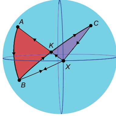
Figure 6.6: Illustrating the generalized solid angle \Omega_{XABC} . In going from state A to state B , the beam acquires a geometric phase equal to half the solid angle \Omega_{XAB} , which is positive. In going from B to C the acquired phase equals half the solid angle \Omega_{XBC} , which is negative. Since the triangle BKX does not contribute, this is equivalent to the generalized solid angle \Omega_{XABC} , which equals half the solid angle of the triangle ABK (positive), plus half the solid angle of the triangle XKC (negative).
