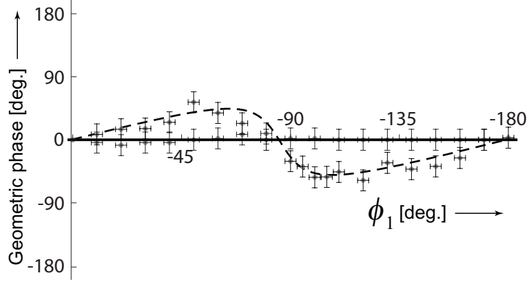
Figure 5.5: Geometric phase of the final state E when the initial state A coincides with the south pole (solid curve), and when A lies between the equator and the south pole (dashed curve), both as a function of the orientation angle \phi_1 . The curves are theoretical predictions [Eq. (5.14)], the dots and error bars represent measurements. In this example \phi_2 = 0 .
