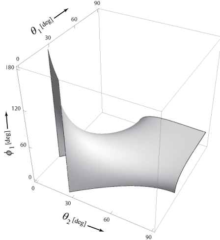
Figure 4.3: A two-dimensional coherence singularity in (\theta_1, \theta_2, \phi_1) -space. In this example k^2 \sigma_S^2 = 10 .
