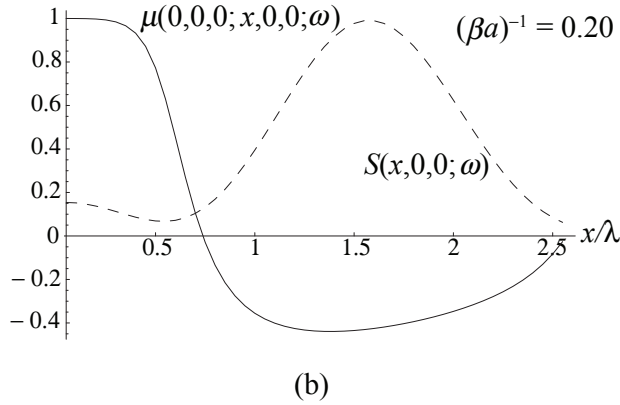
Figure 2.7: Spectral degree of coherence \mu(0,0,0;x,0,0;\omega) (solid line) and the spectral density S(x,0,0;\omega) normalized to its maximum value (dashed line), for the case (a): (\beta a)^{-1} = 0.25 and (b): (\beta a)^{-1} = 0.2 . In this example \lambda = 0.6328 \mu\text{m} , a = 0.01 \text{ m} , and f = 0.02 \text{ m} .
