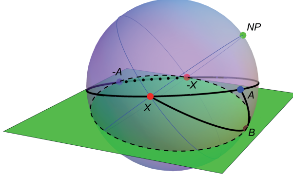
Figure 6.2: Illustrating the intersection of the plane given by Eq. (6.10) and the Poincaré sphere. This intersection is a circle (indicated by the dashed curve) that runs through the points -A , -X and B . All points on the circle segment that runs from -A to B to -X constitute the set \{B'\} of states that have the same phase difference \gamma_{AB} with respect to A as the state B . The great circle through A and X is shown solid-dotted. The point NP indicates the North Pole.
