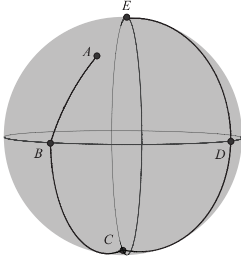
Figure 5.1: Non-closed path ABCDE on the Poincaré sphere for a monochromatic light beam that passes through a sequence of polarizers and compensators.
