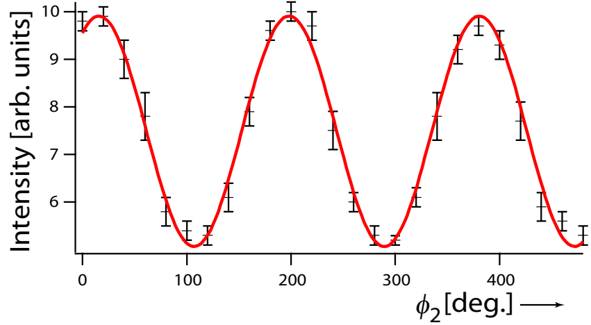
Figure 5.3: Measured intensity as a function of the orientation angle \phi_2 . The solid curve is a fit of the measured data to the function C_1 + C_2 \cos(2\phi_2 + C_3) . The vertical symbols indicate error bars.
