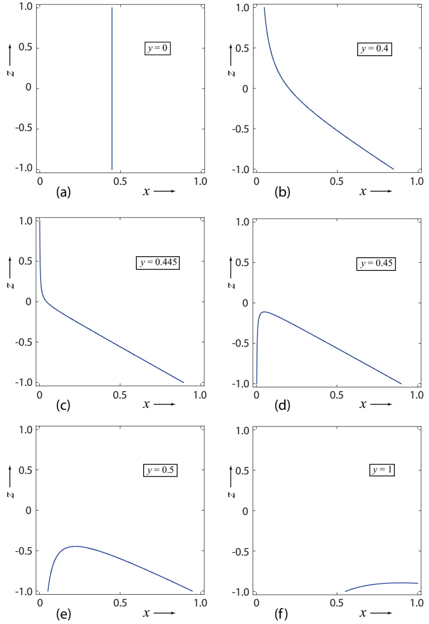
Figure 4.6: Cross-sections of the coherence singularity in the x, z -plane for selected values of y , viz. y = 0 (a), y = 0.4 (b), y = 0.445 (c), y = 0.45 (d), y = 0.5 (e), and y = 1 (f).
