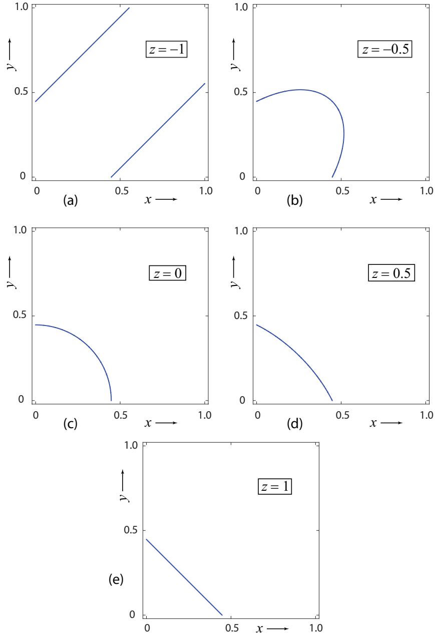
Figure 4.5: Cross-sections of the coherence singularity in the x, y -plane for selected values of z , viz. z = -1 (a), z = -0.5 (b), z = 0 (c), z = 0.5 (d), and z = 1 (e).
