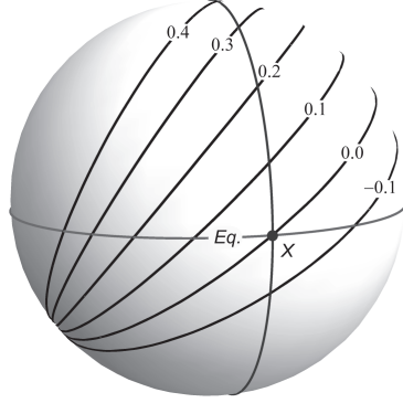
Figure 6.3: Selected contours of the phase \gamma_{AB} for the case \mathbf{A} = (0, 0.8, 0.6) . The basis-state X , the equator ( Eq. ) and the meridian through X are also shown.
