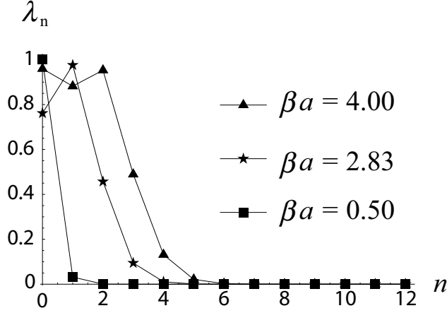
Figure 2.9: Eigenvalues \lambda_n versus n for a J_0 -correlated field with a uniform spectral density across the plane of the aperture. Only the points corresponding to integer values of n are meaningful, the connecting lines are drawn to aid the eye.
