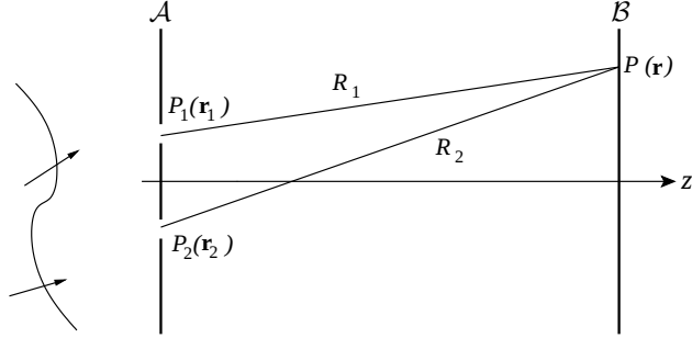
Figure 1.1: Young's interference experiment.
