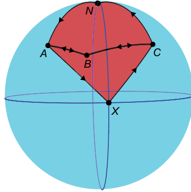
Figure 6.7: Illustrating the equality \Omega_{NABC} + \Omega_{CBAX} = \Omega_{NAXC} . Such a construction can be made for any choice of states.
