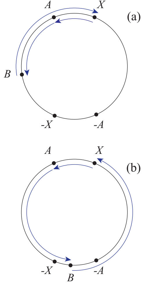
Figure 6.1: The great circle through A , B and basis state X . If state B does not lie on the segment between -A and -X [panel (a)], then the sum of the three geodesics XA , AB and BX is zero. If B lies on the segment between -A and -X [panel (b)], then the sum of the three geodesics equals the great circle.
