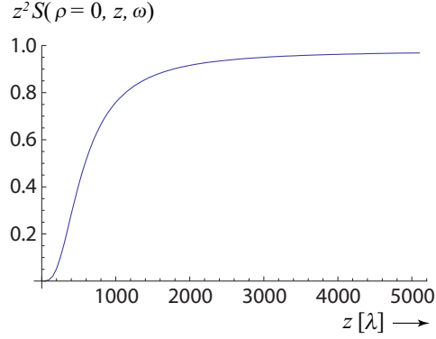
Figure 3.2: The scaled on-axis spectral density z^2 S(\boldsymbol{\rho} = 0, z, \omega) , calculated from Eq. (3.20), normalized by the radiant intensity in the forward direction J[\mathbf{s} = (0, 0, 1), \omega] . In this example \sigma_S = 15\lambda and \sigma_\mu = 4\lambda .
