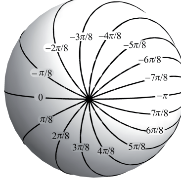
Figure 6.5: Contours of equal phase of \gamma_{AB} for the case that the state A is taken to be (0, 0, 1) . The singularity at -A is seen to have topological charge +1 .
