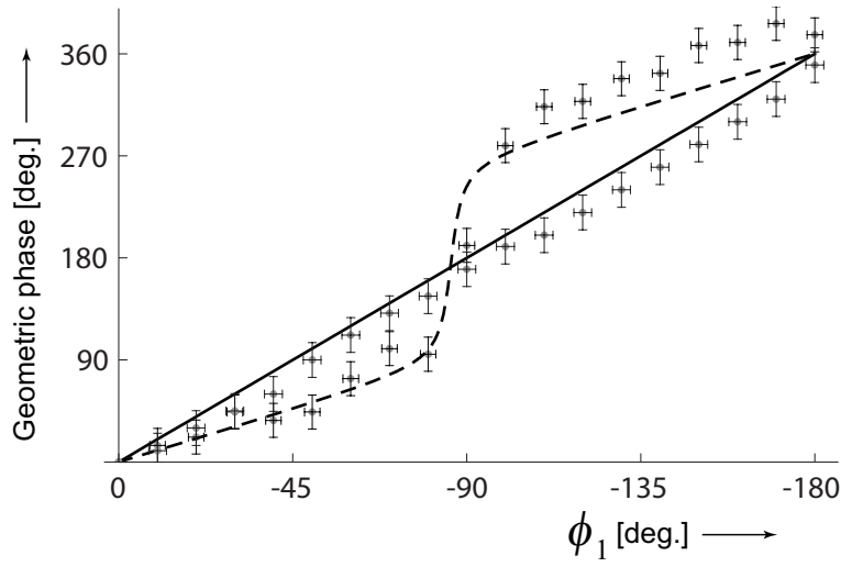
Figure 5.4: Geometric phase of the final state E when the initial state A coincides with the north pole (solid curve), and when A lies between the equator and the north pole (dashed curve), both as a function of the orientation angle \phi_1 . The curves are theoretical predictions [Eq. (5.14)], the dots and error bars represent measurements. In this example \phi_2 = 0 .
