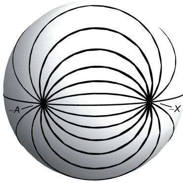
Figure 6.4: Contours of equal phase of \gamma_{AB} for the case that the state A is taken to be (0.6, 0, 0.8) . Two singular points with opposite topological charge can be seen at -A and -X .
