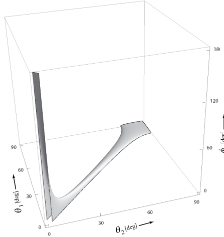
Figure 4.4: A two-dimensional coherence singularity in (\theta_1, \theta_2, \phi_1) -space. In this example k^2 \sigma_S^2 = 1000 .
