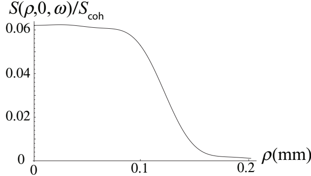
Figure 2.8: Normalized spectral density, Eq. (2.39), in the focal plane for the case (\beta a)^{-1} = 0.13 . In this example \lambda = 500 nm, a = 0.01 m, n = 2 , and f = 2 m.
