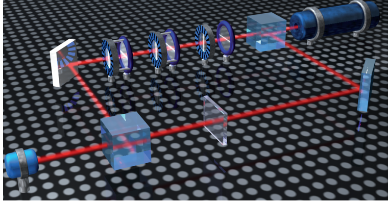
Figure 5.2: Sketch of the Mach-Zehnder setup. The light from a He-Ne laser (right-hand top) is split into two beams. All polarizing elements are placed in the upper arm, the lower arm only contains a gray filter. The compensators are depicted with striped holders, the linear polarizers with non-striped holders. The last two pairs of elements are mounted together. The interference pattern of the recombined beams is recorded with either a photo diode or a CCD camera (left-hand bottom).
