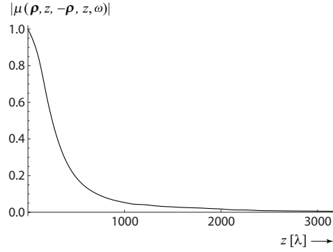
Figure 3.4: Evolution of the modulus of the spectral degree of coherence, as calculated from Eq. (3.18), along the two directions of observation at which a coherence singularity occurs in the far field. In this example \sigma_S = 15\lambda and \sigma_\mu = 4\lambda .
