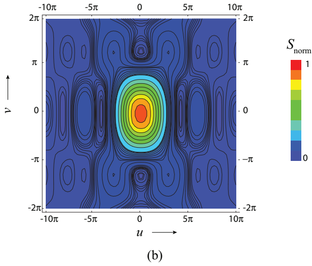
Figure 2.2: The three-dimensional normalized spectral density distribution (a) and its contours (b) for the case \beta^{-1} = 0.02 m, a = 0.01 m and hence (\beta a)^{-1} = 2.00 . In this example \lambda = 500 nm, and f = 2 m.
