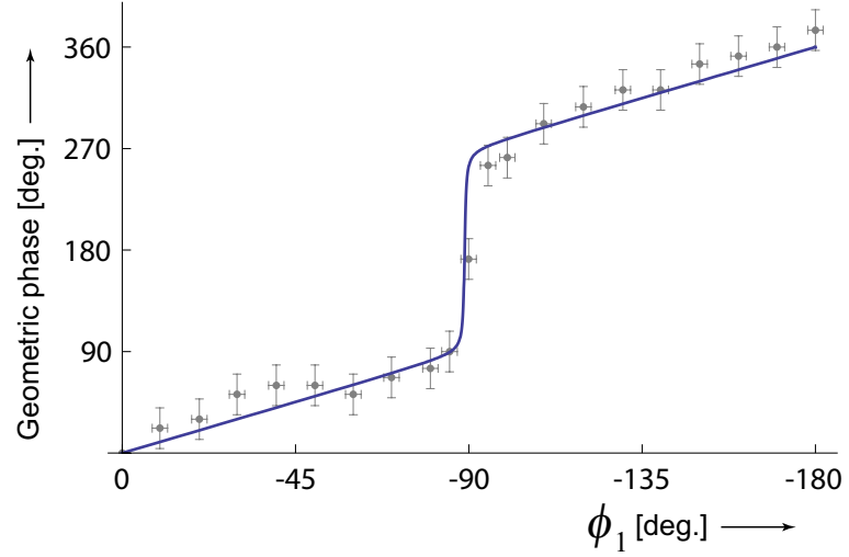
Figure 5.7: Singular behavior of the geometric phase of the final state E when the initial state A lies on the equator, as a function of the orientation angle \phi_1 . The solid curve is a theoretical prediction [Eq. (5.14)], the dots and error bars represent measurements. In this example \theta_A = 0.27 , \alpha_A = 0.0 and \phi_2 = 0 .
