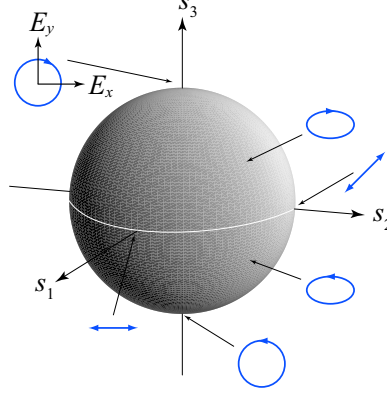
Figure 1.3: The Poincaré sphere with Cartesian axes (s_1, s_2, s_3) .
