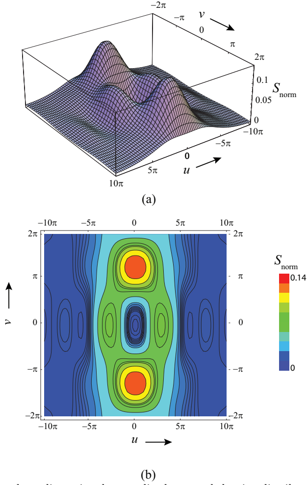
Figure 2.4: The three-dimensional normalized spectral density distribution (a) and its contours (b) for the case \beta^{-1} = 2.5 \times 10^{-3} m, a = 0.01 m and hence (\beta a)^{-1} = 0.25 . The other parameters are the same as those of Fig. 2.2.
