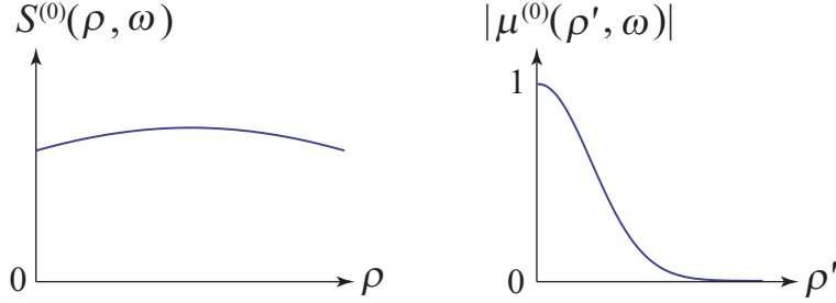
Figure 4.2: Illustrating the concept of quasi-homogeneity.
