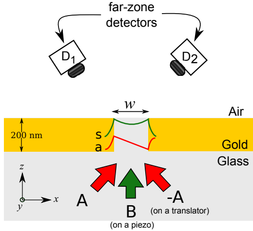
Figure 7.1: A subwavelength slit of width w = 500 nm in a gold film supports only two TM modes for w < \lambda , a symmetric mode (s, green curve) and an anti-symmetric mode (a, red curve). Three coherent beams, A, -A (with opposite angle of incidence compared to A and \pi -phase shifted), and B are incident on the slit from the glass substrate.
