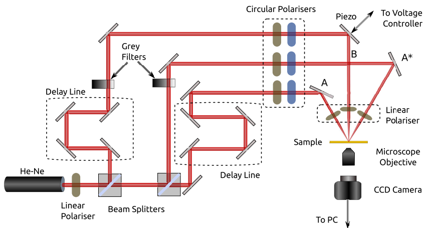
Figure 6.3: Sketch of the experimental setup. The sample is illuminated from the glass-substrate side.
