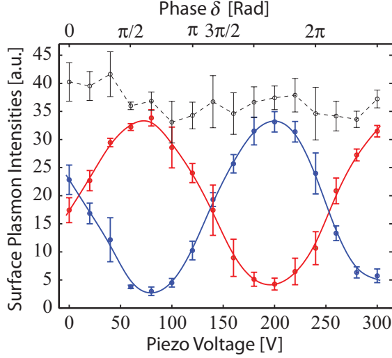
Figure 6.5: Experimental results of the proposed plasmon switching method. The SP intensities I^{(l)}(\delta) (red curve) and I^{(r)}(\delta) (blue curve) are shown as a function of the phase \delta of arm B or, equivalently, as a function of the voltage across the piezo element. The total intensity I^{(l)}(\delta) + I^{(r)}(\delta) is shown as a dotted grey curve. The error bars indicate the standard deviation of ten independent measurements.
