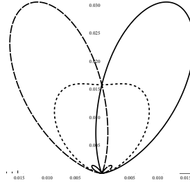
Figure 7.2: The radiation pattern of a sub-wavelength slit for three values of the phase difference \delta . For the dashed curve \delta = -\pi/2 , for the dotted curve \delta = 0 and for the solid curve \delta = \pi/2 .
