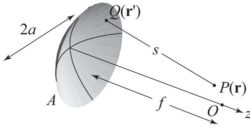
Figure 2.1: Illustration of the focusing configuration.
