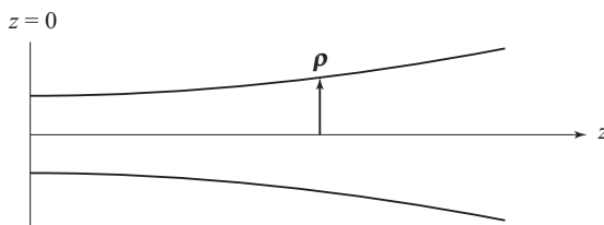
Figure 4.1: Illustrating the notation. The vector \boldsymbol{\rho} = (x, y) indicates a transverse position.
