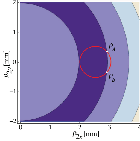
Figure 4.2: The locus of equal modulus of W_{xx} and W_{yy} (red curve), and the contours of \text{Arg}[W_{xx}] - \text{Arg}[W_{yy}] = \pi \pmod{2\pi} . Their intersections, \boldsymbol{\rho}_A and \boldsymbol{\rho}_B , are correlation singularities. In this example A_x = 1 , A_y = 3 , \lambda = 632.8 nm, \sigma = 1 mm, \delta_{xx} = 0.2 mm, \delta_{yy} = 0.09 mm, z = 1.4 m, and \boldsymbol{\rho}_1 = (2.5, 0) mm.
