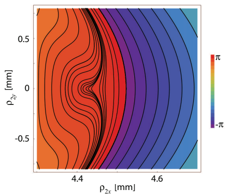
Figure 5.16: Phase contours of \eta(\boldsymbol{\rho}_1, \boldsymbol{\rho}_2, z) in the plane z = 3.33 m, right after the final topological reaction. There are no more singularities or stationary points.
