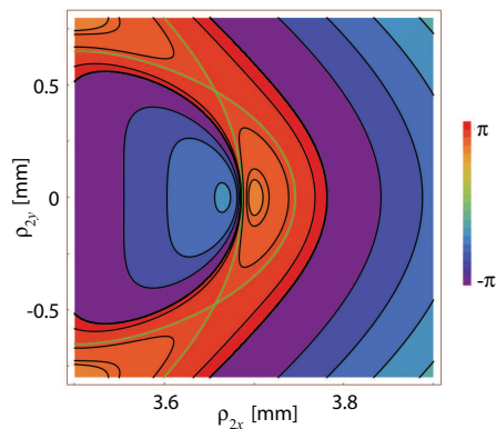
Figure 5.14: Phase contours of \eta(\boldsymbol{\rho}_1, \boldsymbol{\rho}_2, z) in the plane z = 2.4 m, containing a maximum, a minimum and two saddle points (intersections of the green curves).
