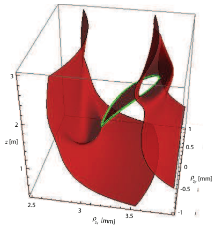
Figure 5.5: Two surfaces for which the phase of \eta(\boldsymbol{\rho}_1, \boldsymbol{\rho}_2, z) equals \pi . In this case \delta_{yy} = 0.12 mm. A closed string of coherence vortices (green curve) has come into existence. The right-hand phase sheet terminates on the string, creating a hole and a protrusion of the sheet.
