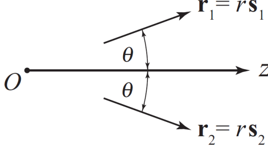
Figure 3.2: Two symmetrically located observation points, with \mathbf{s}_{1\perp} = -\mathbf{s}_{2\perp} .
