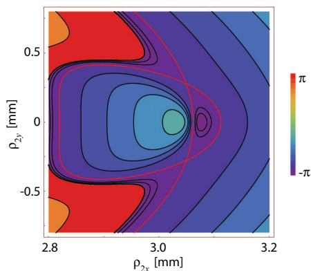
Figure 5.11: Phase contours of \eta(\boldsymbol{\rho}_1, \boldsymbol{\rho}_2, z) in the plane z = 1.12 m. The right-hand side phase saddle of Fig. 5.8 has decayed into a minimum and two saddles (intersections of the two red curves).
