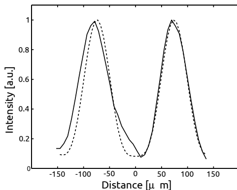
Figure 2.8: Intensity distribution in the focal plane for an iris of radius 1.2mm
