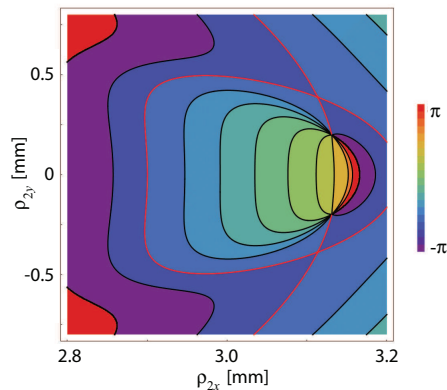
Figure 5.13: Phase contours of \eta(\boldsymbol{\rho}_1, \boldsymbol{\rho}_2, z) in the plane z = 1.4 m, containing two vortices (“coherence singularities”) and two saddle points (intersections of the red curves).
