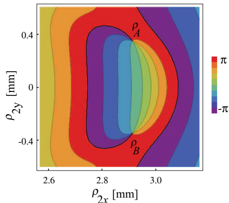
Figure 4.3: Color-coded phase plot of the degree of coherence \eta(\boldsymbol{\rho}_1, \boldsymbol{\rho}_2, z) in the plane z = 1.4 m. The singularities at \boldsymbol{\rho}_A and \boldsymbol{\rho}_B have opposite topological charge.
