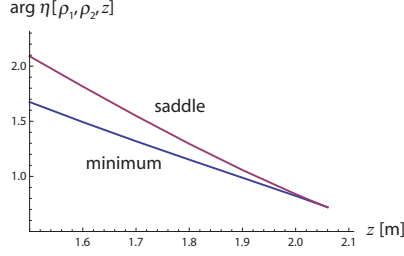
Figure 5.9: Phase of \eta(\boldsymbol{\rho}_1, \boldsymbol{\rho}_2, z) at the minimum and at the phase saddle (visible on the left-hand side in Fig. 5.8), in various cross-sections of the beam.
