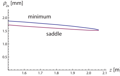
Figure 5.10: The position \rho_{2x} of the minimum (blue curve) and that of the saddle (red curve) in various cross-sections of the beam. Near z = 2.06 m the minimum and the saddle point annihilate each other.
