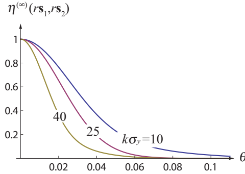
Figure 3.4: The spectral degree of coherence of a beam generated by a quasi-homogeneous source in the far field. The two symmetrically located observation points each make an angle \theta with the beam axis (see Fig. 3.2). The normalized widths of the two spectral densities are k\sigma_x = 20 and k\sigma_y = 10, 25, 40 .
