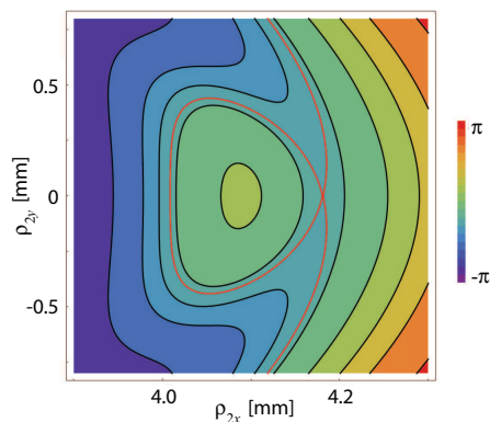
Figure 5.15: Phase contours of \eta(\boldsymbol{\rho}_1, \boldsymbol{\rho}_2, z) in the plane z = 3.0 m, containing a maximum and a saddle (intersection of the red curve).
