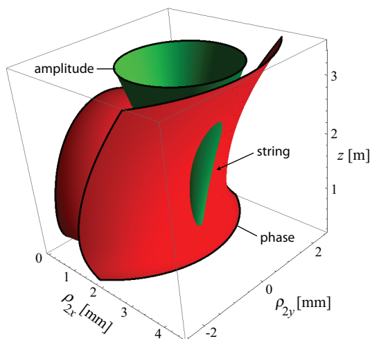
Figure 4.5: The intersection of a surface of equal amplitude (green) and a surface of opposite phase (red) constitutes a string of correlation singularities.
