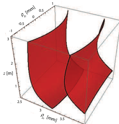
Figure 5.2: Two surfaces for which the phase of \eta(\boldsymbol{\rho}_1, \boldsymbol{\rho}_2, z) equals \pi . In this case \delta_{yy} = 0.18 mm. The other parameters are \lambda = 632.8 nm, \delta_{xx} = 0.2 mm, \sigma = 1 mm, A_x = 1 and A_y = 3 . The reference point \boldsymbol{\rho}_1 = (2.5, 0) mm.
