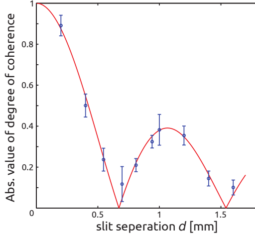
Figure 2.3: Modulus of the degree of spatial coherence of the field as a function of the slit separation d . The solid line indicates the theoretical prediction, the circles indicate experimental values with error bars.
