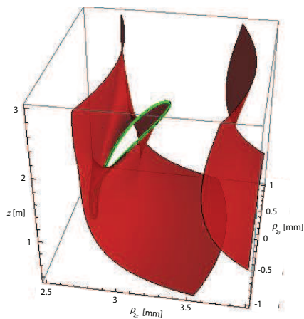
Figure 5.6: A single surface for which the phase of \eta(\rho_1, \rho_2, z) equals \pi . In this case \delta_{yy} = 0.11 mm. The string of coherence vortices (green curve) has expanded, causing the protrusion of Fig. 5.5 to grow. The two formerly disjoint phase sheets are now connected.
