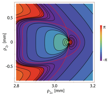
Figure 5.12: Phase contours of \eta(\boldsymbol{\rho}_1, \boldsymbol{\rho}_2, z) in the plane z = 1.1808 m, containing a dipole and two saddle points (intersections of the red curves).
