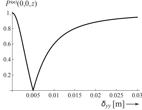
Figure 3.5: The spectral degree of polarization of a beam generated by a quasi-homogeneous source at a far-field axial point. In this example one effective coherence length is taken to be \delta_{xx} = 0.5 cm, whereas \delta_{yy} = varies between 0 and 3 cm. The two spectral densities S_x^{(0)} and S_y^{(0)} are assumed to be equal.
