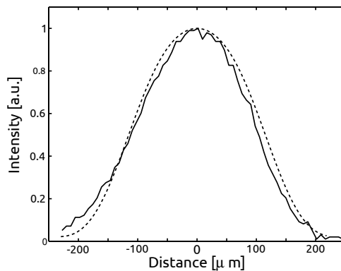
Figure 2.6: Intensity distribution in the focal plane for an iris of radius 0.25mm
