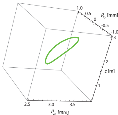
Figure 5.4: A closed string of coherence singularities (green curve).
