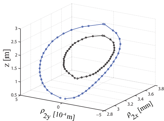
Figure 4.6: Two strings of correlation singularities in a partially coherent beam. The larger string (blue) is for \delta_{yy} = 0.09 mm, the shorter string (black) is for the case \delta_{yy} = 0.12 mm.
