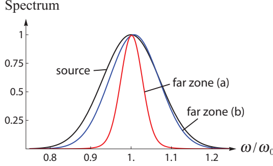
Figure 3.3: The on-axis spectrum in the source plane (black curve), and two on-axis spectra in the far zone. All spectra are normalized to unity. In this example a = 1 , b = 2a , \delta_{xx} = 1 , \delta_{yy} = 2 , \Delta = \omega_0/10 , \Delta_{xx} = 0.1 and \Delta_{yy} = 0.04 [far-zone spectrum (a)] or 0.2 [far-zone spectrum (b)].
