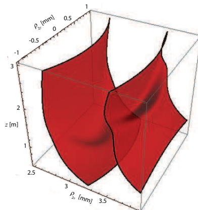
Figure 5.3: Two surfaces for which the phase of \eta(\boldsymbol{\rho}_1, \boldsymbol{\rho}_2, z) equals \pi . In this case \delta_{yy} = 0.14 mm.
