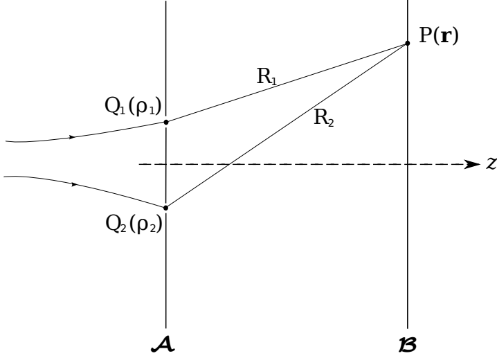
Figure 1.1: Notation pertaining to Young's double slit experiment with a stochastic electromagnetic beam. The two apertures in screen \mathcal{A} are located at \boldsymbol{\rho}_1 and \boldsymbol{\rho}_2 . The observation point P(\mathbf{r}) is on a second, parallel screen \mathcal{B} .
