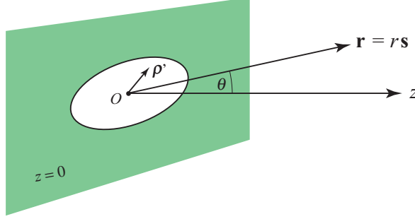
Figure 3.1: Illustrating the notation. The vector \boldsymbol{\rho}' = (x, y) indicates a transverse position in the source plane z = 0 . The line from the origin O to an observation point \mathbf{r} = r\mathbf{s} , with |\mathbf{s}| = 1 , makes an angle \theta with the positive z -axis.
