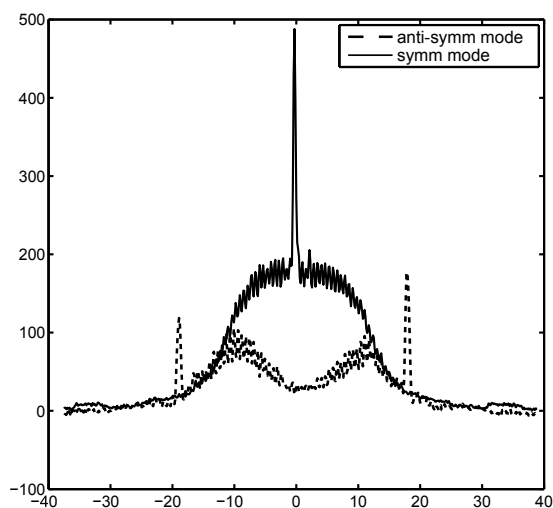
Figure 7.3: Plot of the radiation from a symmetric (blue curve) and an anti-symmetric (red curve) mode.
