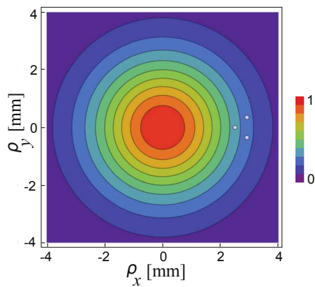
Figure 4.4: Normalized spectral density of the beam in the cross-section z = 1.4 m. The points \boldsymbol{\rho}_1 , \boldsymbol{\rho}_A , and \boldsymbol{\rho}_B are indicated by the three white dots.
