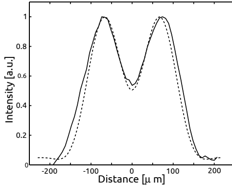
Figure 2.7: Intensity distribution in the focal plane for an iris of radius 0.75mm
