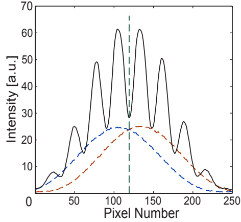
Figure 2.4: Illustration of negative correlation of the field at the two slits. At the center of the fringe pattern (vertical dashed line) an intensity minimum is observed. The dashed lines represent measurements with one slit covered.
