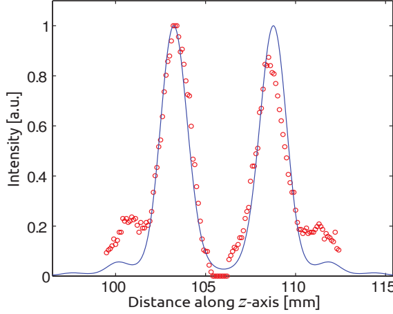
Figure 2.5: Intensity along the z -axis. The solid line represents the theoretical prediction, the circles correspond to experimental measurements.
