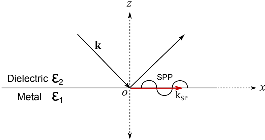
Figure 1.2: The interface between a metal of permittivity \epsilon_1 and a dielectric of permittivity \epsilon_2 .
