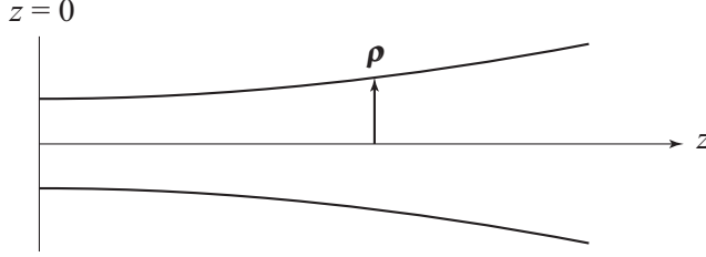
Figure 5.1: Illustrating the notation. A partially coherent, electromagnetic Gaussian-Schell model beam propagates in the z -direction. The source plane is taken to be at z = 0 . The vector \boldsymbol{\rho} = (x, y) indicates a transverse position.
