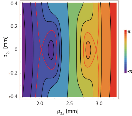
Figure 5.8: Phase contours of \eta(\boldsymbol{\rho}_1, \boldsymbol{\rho}_2, z) in the plane z = 0.1 m. A minimum, a maximum and two saddle points (intersections of the red curves) can be seen. In this and in the following examples we have taken \boldsymbol{\rho}_1 = (2.5, 0) mm, A_x = 1 , A_y = 3 , \sigma = 1 mm, \delta_{xx} = 0.2 mm, \delta_{yy} = 0.12 mm, and the wavelength \lambda = 633 nm.
