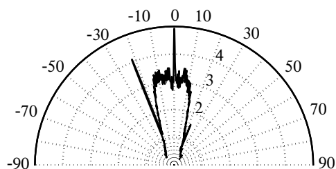
Figure 7.5: (Colour online) Polar plot of light diffracted from the sub-wavelength aperture. The radial scale indicates the intensity (a.u.). The peak of the diffracted light is at an angle on 0^\circ
