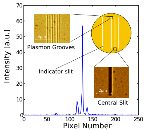
Figure 6.4: Typical line trace of the CCD camera screen, perpendicular to the slits
