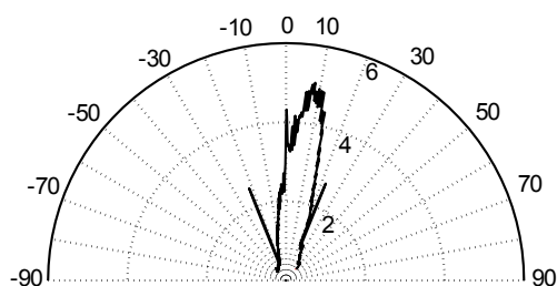
Figure 7.6: (Color online) Polar plot of light diffracted from the subwavelength aperture. The radial scale indicates the intensity (a.u.). The peak of the diffracted light is towards right at an angle of +10^\circ
