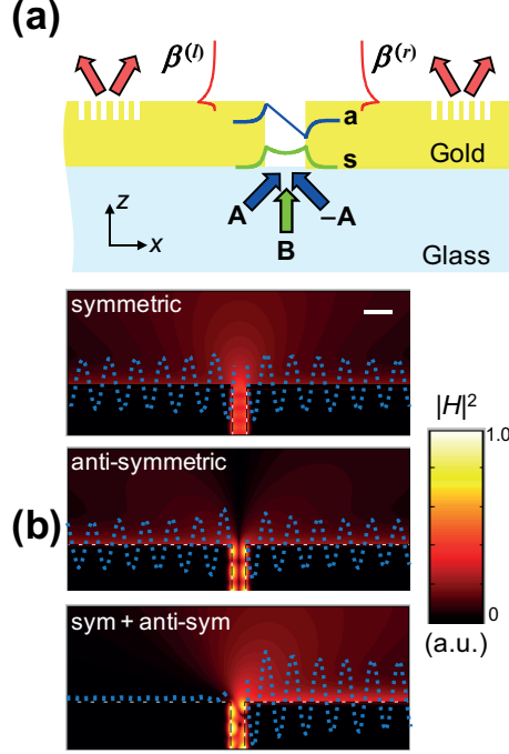
Figure 6.1: Principle of the proposed surface plasmon steering method. (a) A subwavelength slit of width w in a gold film supports only two TM modes for \lambda/2 \lesssim w \lesssim \lambda : a symmetric mode (s, green curve) and an anti-symmetric mode (a, blue curve). Three coherent beams, A, -A (with opposite angle of incidence compared to A and \pi -phase shifted), and B are incident on the slit from the glass substrate. (b) Illustrating how a coherent superposition of the a and s modes can lead to unidirectional SP launching at a gold-air interface. The first two panels show the intensity of the magnetic field when the slit is illuminated with either the s or the a mode. Superposed dotted blue curves show the total magnetic field scattered on the interface. The length of the white bar in the first panel indicates the illumination wavelength in vacuum ( \lambda = 600 nm), and the slit width w is \lambda/2 .
