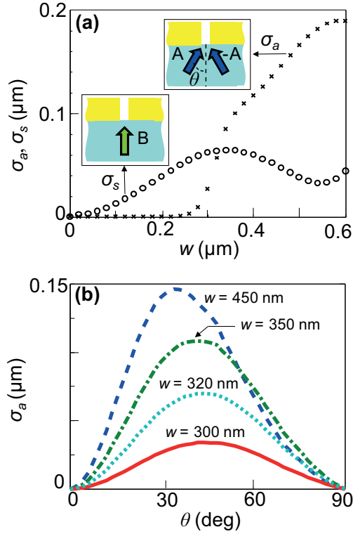
Figure 6.2: The calculated SP cross sections \sigma_a and \sigma_s as defined in Eqs. (6.3) and (6.4) for a unit Poynting vector of each of the incident beams. (a) Variation of \sigma_a and \sigma_s with slit width w . The angles of incidence of the plane waves A, -A are taken to be \theta = \pm 30^\circ . The two insets indicate the setup for calculating \sigma_a and \sigma_s , respectively. (b) Variation of \sigma_a with angle of incidence \theta for slit widths w = 300, 320, 350 , and 450 nm. The refractive index of gold n_{\text{Au}} = 0.18 + i2.99 for \lambda = 632.8 nm, is taken from [PALIK, 1998], and the thickness of the gold film is 200 nm.
