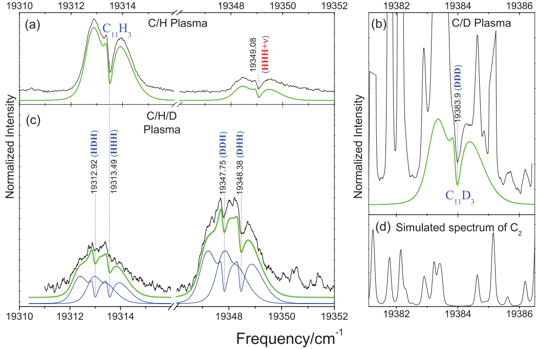
Figure 4.3 – Experimentally observed spectra (upper black lines) of C_{11}H_3 and its D-isotopologues recorded through (a) C/H, (b) C/D, and (c) C/H/D plasma. The simulated spectra are represented by bold green lines. In panel (c), the individual simulations of the observed \alpha -type bands are shown by blue lines. The spectrum in panel (d) consists of simulated rotational lines of C_2 which overlap with the electronic origin band of C_{11}D_3 .
