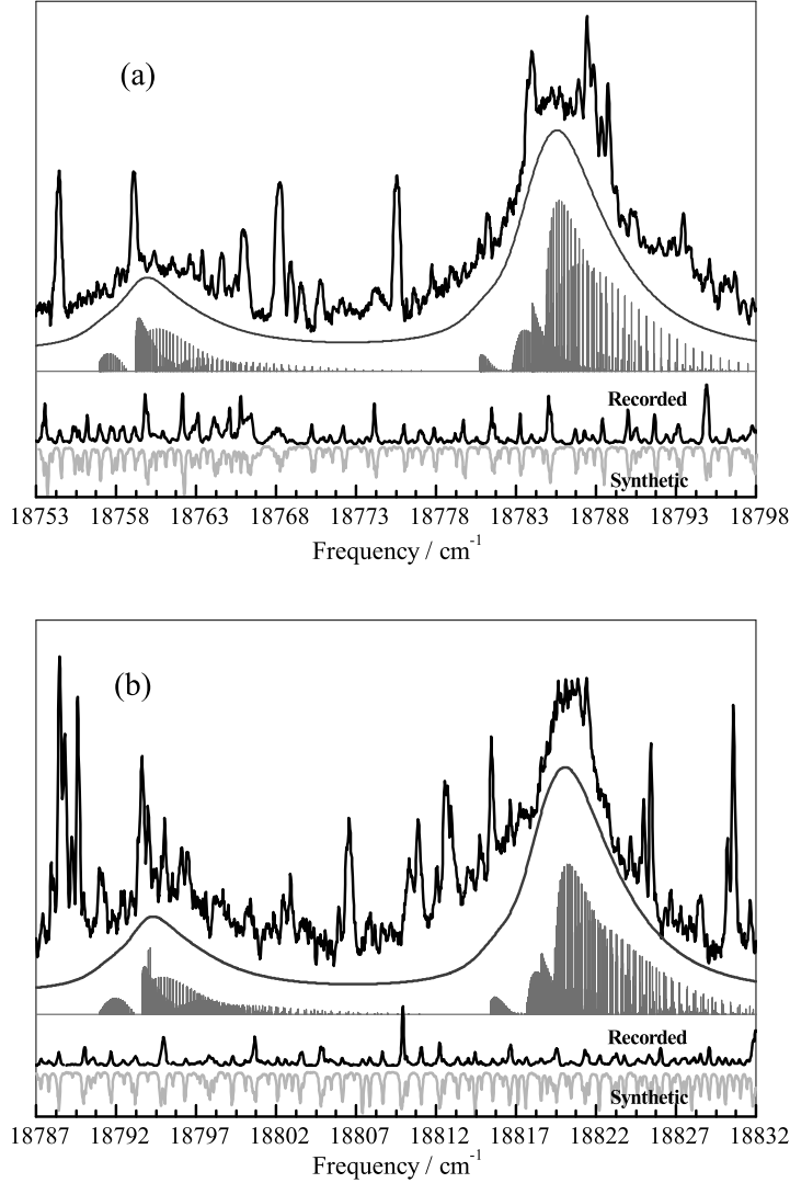
Figure 3.1 – \tilde{A}^2\Delta - \tilde{X}^2\Pi origin band spectra for (a) C 5 H and (b) C 5 D. The upper traces in both panels show the cavity ring-down recordings using a pinhole nozzle. The sharp features in the observed spectra are due to overlapping absorptions of small radicals. The middle traces are the simulated spectra for a Lorentzian line width of \Gamma = 3.3 \text{ cm}^{-1} and a Gaussian line width of 0.12 \text{ cm}^{-1} assuming a rotational temperature of 30 K. The stick diagrams are simulations for a \tilde{A}^2\Delta - \tilde{X}^2\Pi transition using the molecular parameters listed in Table 3.1. The simultaneously recorded I 2 reference spectra are also shown in the lower traces of both panels and matched to the synthetic I 2 spectrum for absolute frequency calibration.
