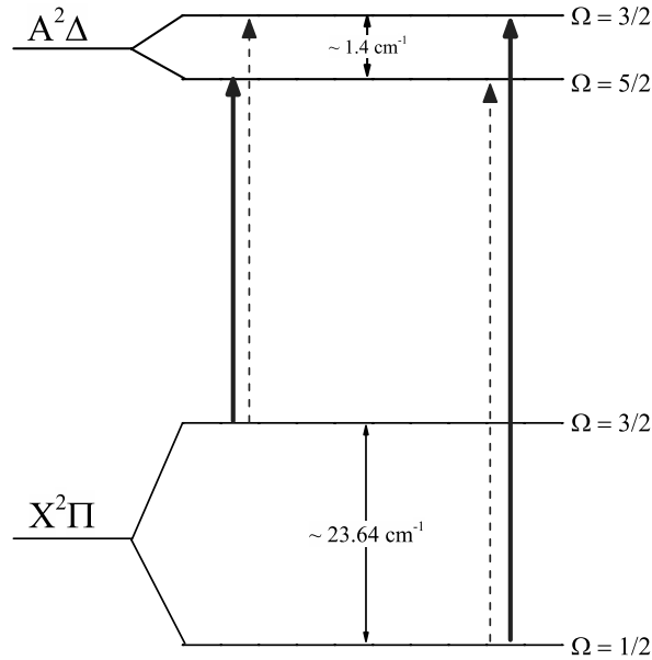
Figure 3.3 – Schematic energy level diagram for the \tilde{X}^2\Pi and \tilde{A}^2\Delta electronic states of \text{C}_5\text{H} . Solid-line arrows indicate the observed \tilde{A}^2\Delta_{3/2} - \tilde{X}^2\Pi_{1/2} and \tilde{A}^2\Delta_{5/2} - \tilde{X}^2\Pi_{3/2} bands. The dashed arrows represent the intrinsically weak (and not observed) \tilde{A}^2\Delta_{5/2} - \tilde{X}^2\Pi_{1/2} and \tilde{A}^2\Delta_{3/2} - \tilde{X}^2\Pi_{3/2} transitions.
