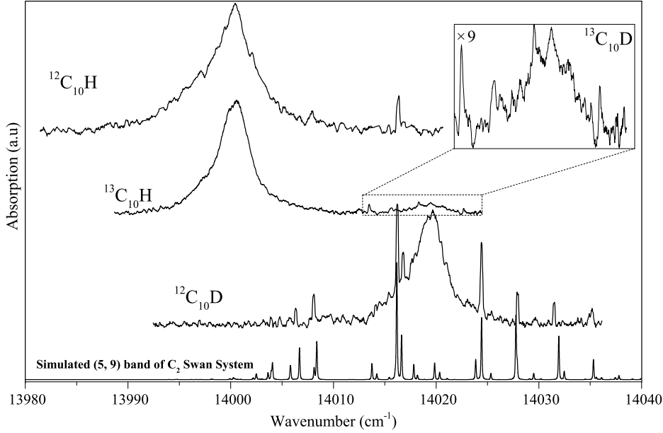
Figure 7.3 – The {}^2\Pi - \tilde{X}{}^2\Pi electronic origin band transition of \text{C}_{10}\text{H} (upper trace), {}^{13}\text{C}_{10}\text{H} (middle trace) and \text{C}_{10}\text{D} (lower trace) observed by cavity ring down spectroscopy in a pulsed pinhole jet plasma. The \text{C}_{10}\text{H} and \text{C}_{10}\text{D} spectra are partially blended with sharp absorption lines of \text{C}_2 as can be concluded from the simulated spectrum of the (5,9) band of the \text{C}_2 Swan system.
