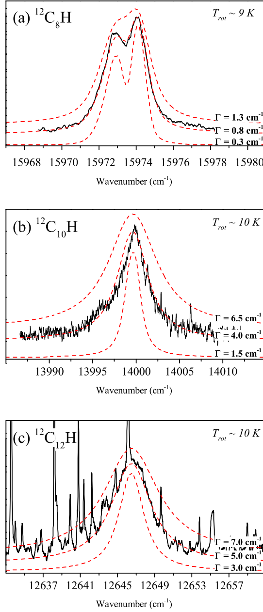
Figure 7.7 – Recorded spectrum of the {}^2\Pi - \tilde{X}^2\Pi electronic origin band transition of \text{C}_8\text{H} (panel a), \text{C}_{10}\text{H} (panel b) and \text{C}_{12}\text{D} (panel c). Simulated spectra for different Lorentzian line width values are shown in each panel.
