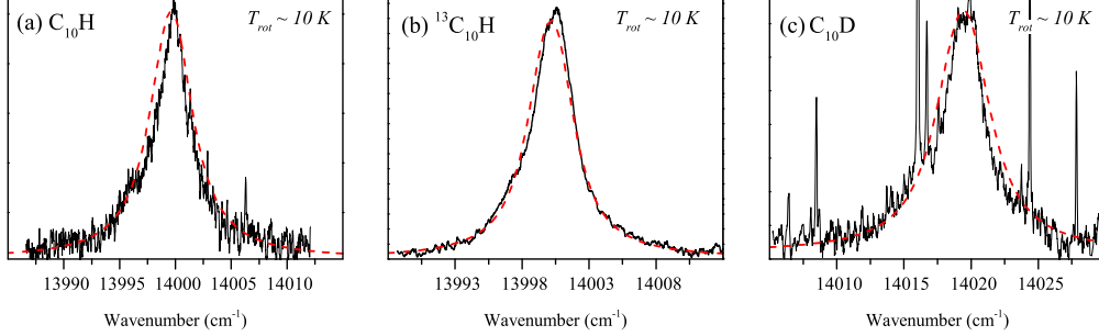
Figure 7.4 – The cold spectra for the three band systems shown in Fig. 7.3. The result of the contour plot fits for T_{rot} = 10 K is incorporated in red, using the constants listed in Table. 7.1.
