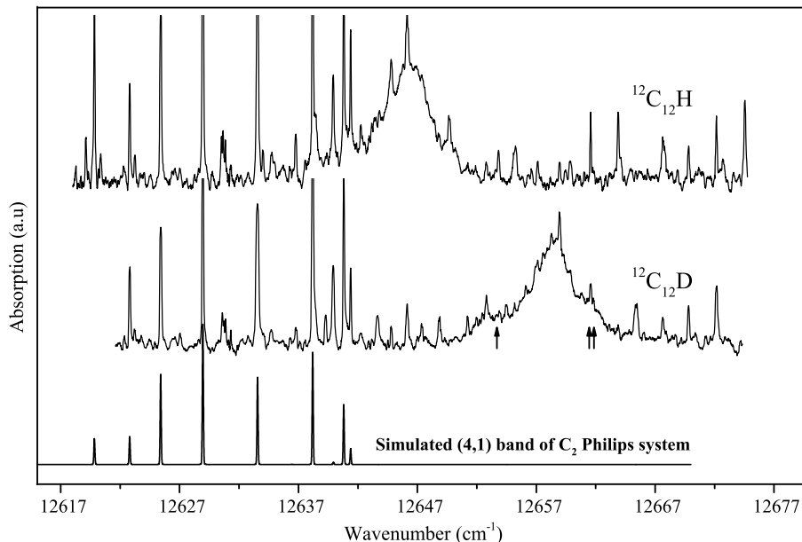
Figure 7.5 – The {}^2\Pi - \tilde{X}{}^2\Pi electronic origin band transition of \text{C}_{12}\text{H} (upper trace) and \text{C}_{12}\text{D} (lower trace) observed by cavity ring down spectroscopy in a pulsed pinhole jet plasma. The origin of the side-bands to the main peak in the \text{C}_{12}\text{D} spectrum, marked by arrows, is unknown (see text). Polluting transitions are due to (4, 1) band transitions of the \text{C}_2 Philips system as simulated in red.
