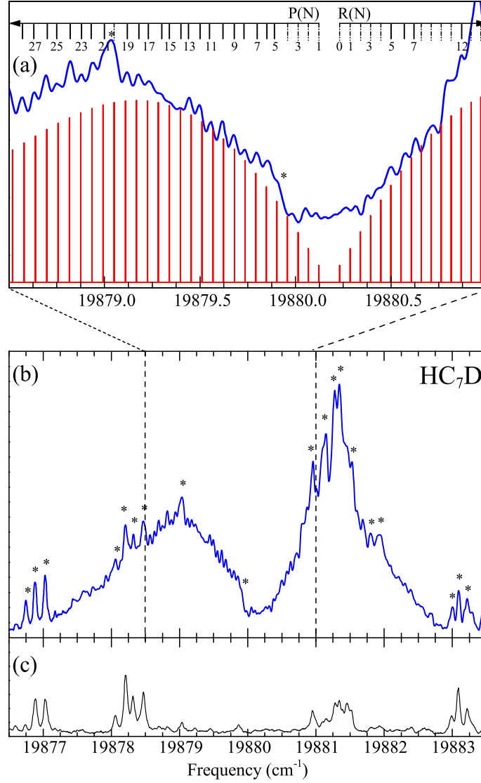
Figure 5.1 – (a) The expanded spectrum of the \tilde{A}^3\Sigma_u^- - \tilde{X}^3\Sigma_g^- electronic transition of \text{HC}_7\text{D} (upper trace) in the band origin region compared with a simulated stick diagram using an effective ^1\Sigma - ^1\Sigma Hamiltonian. The full spectrum is shown in panel (b). Peaks due to overlapping spectra originating from other species are marked by an asterisk and shown in panel (c) for expansion conditions not in favor of carbon chain formation.
