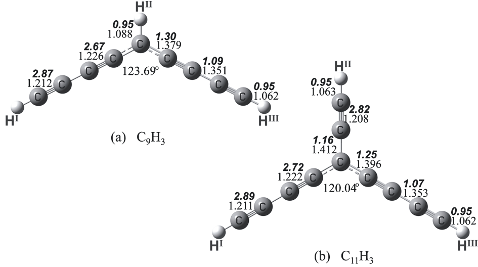
Figure 4.1 – The molecular structure of (a) \text{C}_9\text{H}_3 and (b) \text{C}_{11}\text{H}_3 . The bond lengths (in Angstrom) and the angles of the bend C_{2v} structures, calculated at the DFT-B3LYP/6-311G** level, are indicated by regular numbers. The calculated bond indices of the two radicals are indicated by bold numbers.
