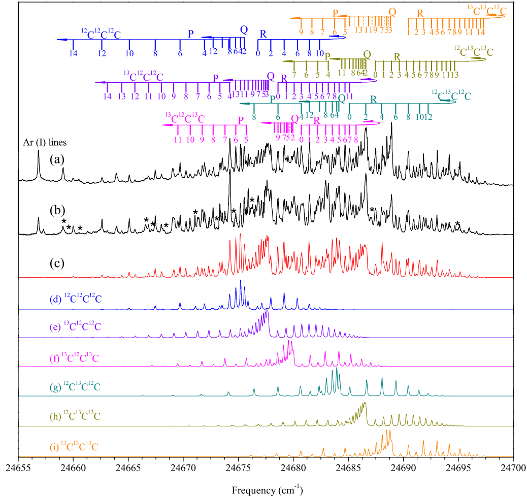
Figure 6.3 – The six blended spectra of the \tilde{A}^1\Pi_u - \tilde{X}^1\Sigma_g^+ 000 - 000 bands of the ^{12}C_3 and ^{13}C -substituted C_3 radicals in a mixed ( ^{13}C_2H_2 + ^{12}C_2H_2 )/He/Ar plasma, with (a) the ratio of ^{12}C/^{13}C < 1 and (b) of ^{12}C/^{13}C > 1 . The Ar(I) absorption line [181] has been used for absolute calibration of the recorded spectra. The red trace (c) shows a weighted sum of simulated spectra, based on simulated spectra for the individual isotopologues (shown in (d) to (i) traces), using a Lorentzian line width of 0.07\text{ cm}^{-1} , a Gaussian line width of 0.1\text{ cm}^{-1} , and a rotational temperature of \sim 40\text{ K} . The P-, Q- and R-branches of the observed rotational lines for the isotopologues are indicated. The lines marked with an asterisk are due to blending transitions of other small species or unknown perturbation features.
