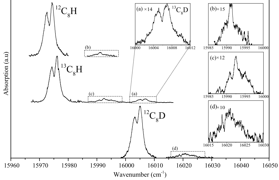
Figure 7.1 – The {}^2\Pi - \tilde{X}^2\Pi electronic origin band transition of \text{C}_8\text{H} (upper trace), {}^{13}\text{C}_8\text{H} (middle trace) and \text{C}_8\text{D} (lower trace) observed by cavity ring down spectroscopy in a pulsed pinhole jet plasma. The weak origin band of the {}^2\Pi - \tilde{X}^2\Pi electronic transition of {}^{13}\text{C}_8\text{D} is shown in panel (a) and an unstructured component of a sequence transition of the lowest frequency bending mode is shown in panels (b), (c) and (d) for \text{C}_8\text{H} , {}^{13}\text{C}_8\text{H} and \text{C}_8\text{D} , respectively.
