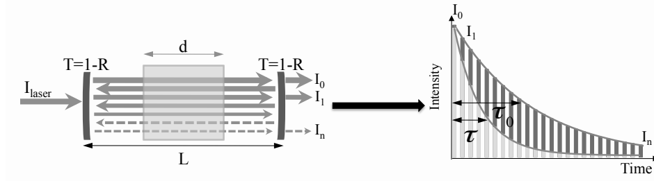
Figure 2.1 – Basic principle of cavity ring down spectroscopy.
