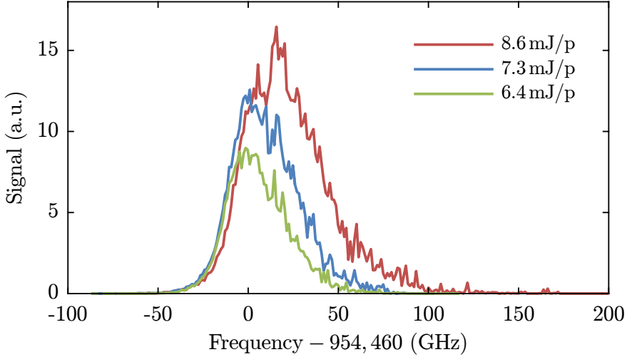
Figure 3.6 – 3+1 REMPI spectra at frequencies around the 3s^2 3p^5(^1S) to 3s^2 3p^5(^2P_{1/2})4s -transition in argon.
