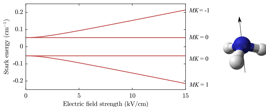
Figure 1.3 — Left: Stark shifts of the sublevels of the J = 1 ro-vibrational ground state of ND 3 as a function of electric field strength [8]. Right: schematic representation of an ammonia molecule including its three-fold rotational symmetry axis.
