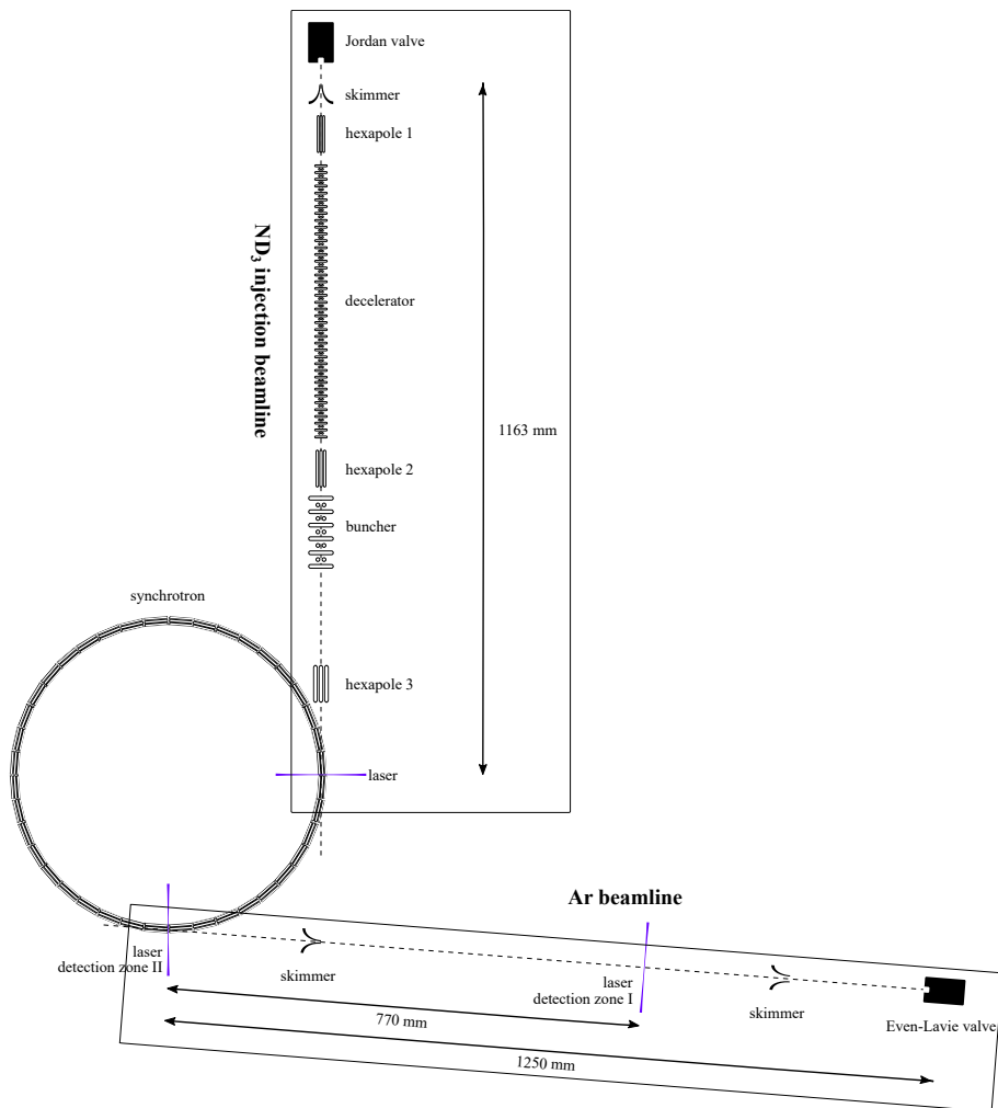
Figure 3.3 – Top view of the experimental set-up (to scale). ND 3 molecules are decelerated to velocities of 100–150 m/s using a Stark decelerator and injected into a molecular synchrotron consisting of 40 electric hexapole elements arranged in a half-meter-diameter circle. Ammonia molecules can be detected at the injection point or at a quarter ring downstream (detection zone II). The argon beamline consists of a cooled solenoid valve that is skimmed by a 5 mm and a 1.5 mm skimmer. Argon atoms are detected 770 mm in front of the synchrotron (detection zone I) or inside the synchrotron (detection zone II). The argon beamline makes an angle of 94,5 degrees with respect to the injection beamline such that the argon beam moves parallel to the first hexapole in the synchrotron behind detection zone II.
