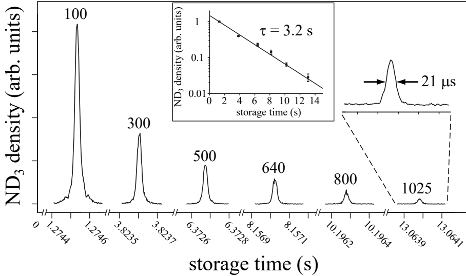
Figure 3.4 — Time-of-flight measurements of ammonia molecules traversing the synchrotron. The numbers above the peaks denote the number of round-trips the molecules have completed at the time of measurement. The inset shows that the 1/e trapping time is 3.2 s. Reprinted with permission from Ref. [56] ©2010 APS.
