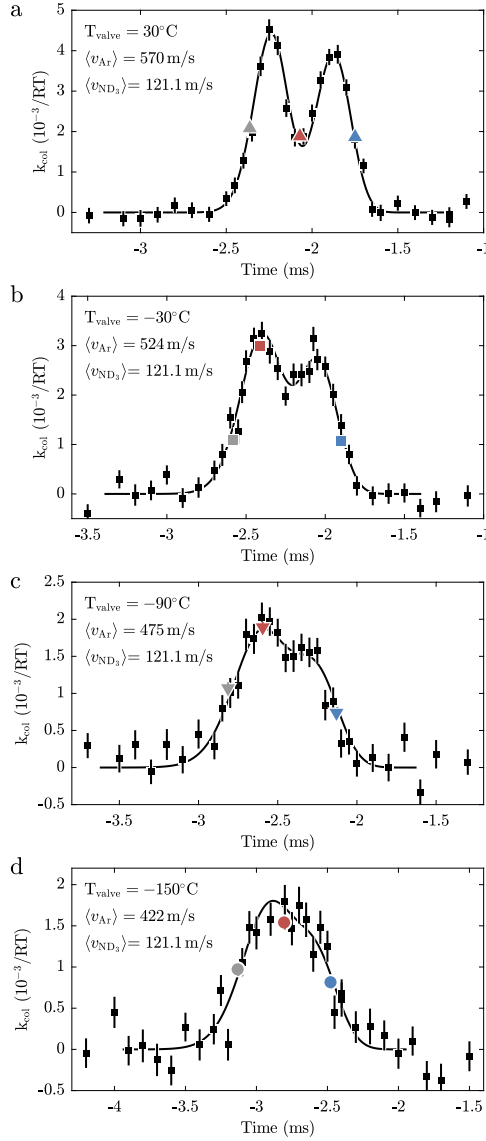
Figure 3.16 – Measured loss rate as a function of the delay between the trigger of the valve and the arrival time of the ammonia packets at the detection zone, for v_{\text{ND}_3} = 121.1 \text{ m/s} . Panels a–d depict measurements with different temperatures of the valve housing that result in different average velocities, as indicated in the top left corners. The black squares represent measurements containing 2400 shots each, while the coloured points represent measurements containing 21,600 shots each. The error bars, for the coloured points obscured by the symbols, denote the standard errors. The black lines show the results of simulations described in Section 3.5.2, scaled to fit the data in each panel. The reduced \chi^2 s of the fits are 0.93, 1.01, 1.09, and 1.31 for panels a–d, respectively.
