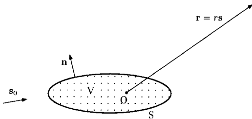
Fig. 1. A plane wave, propagating along the direction of the unit vector s_0 , is incident on a scattering volume V . The volume is bounded by a closed surface S , with outward unit normal \mathbf{n} . The direction of scattering is denoted by s .
