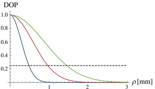
Fig. 2. Degree of polarization (DOP) in the back focal plane of a lens as a function of the radial distance \rho . The dashed horizontal line indicates |B_{xy}| , the modulus of the DOP in the front focal plane. In this example, \lambda = 632.8 nm, f = 1 m (blue curve), f = 2 m (red curve), or f = 3 m (green curve), B_{xy} = 0.25 , \sigma = 5 mm, \delta = 0.2 mm, and \delta_{xy} = 0.4 mm.
