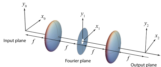
Fig. 3. 4f setup for Fourier processing consisting of two identical lenses with focal length f . An iris with radius a is situated in the Fourier plane.
