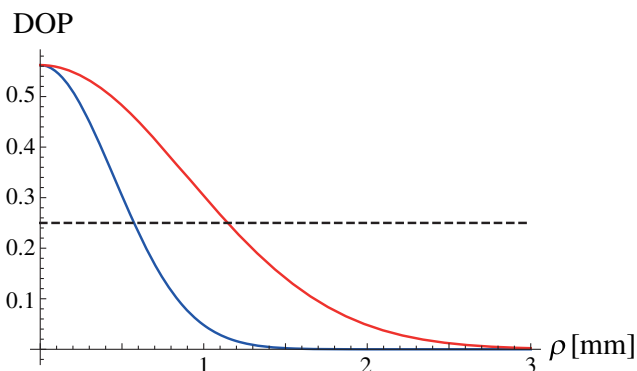
Fig. 1. Degree of polarization (DOP) in the back focal plane of a lens as a function of the radial distance \rho . The dashed horizontal line indicates |B_{xy}| , the modulus of the DOP in the front focal plane. In this example, \lambda = 632.8 nm, f = 1 m (blue curve) or f = 2 m (red curve), B_{xy} = 0.25 , \sigma = 5 mm, \delta = 0.2 mm, and \delta_{xy} = 0.3 mm.
