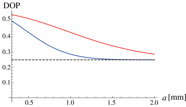
Fig. 4. Degree of polarization in the output plane as a function of the aperture radius a for f = 1 m (blue) and f = 2 m (red). The DOP in the input plane is indicated by the dashed horizontal line. All other parameters are defined in Fig. 1.
