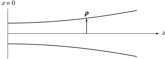
Fig. 1. Illustrating the notation. The vector \rho = (x, y) indicates a transverse position.
