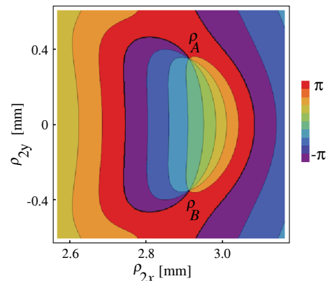
Fig. 3. (Color online) Color-coded phase plot of the degree of coherence \eta(\rho_1, \rho_2, z) in the plane z = 1.4 m. The singularities at \rho_A and \rho_B have opposite topological charge.
