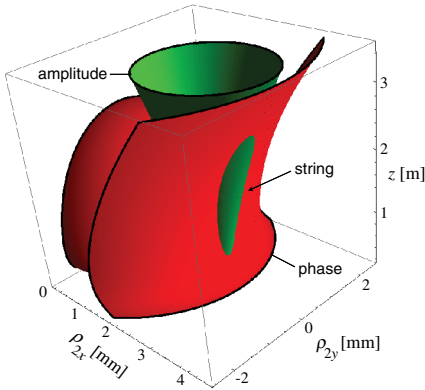
Fig. 5. (Color online) Intersection of a surface of equal amplitude (green) and a surface of opposite phase (red) constitutes a string of correlation singularities.
