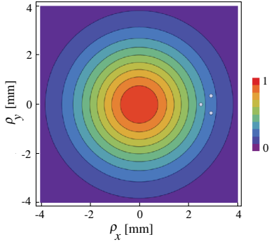
Fig. 4. (Color online) Normalized spectral density of the beam in the cross section z = 1.4 m. The points \rho_1 , \rho_A , and \rho_B are indicated by the three white dots.
