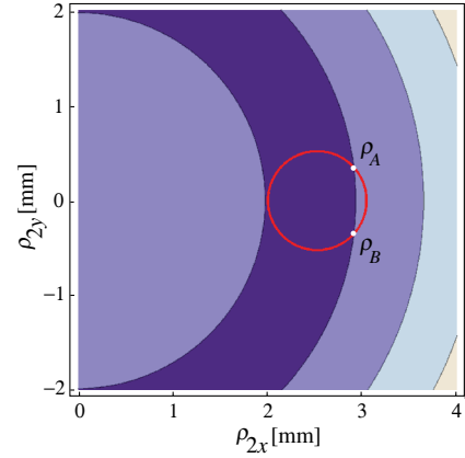
Fig. 2. (Color online) Locus of equal modulus of W_{xx} and W_{yy} (red curve), and the contours of \text{Arg}[W_{xx}] - \text{Arg}[W_{yy}] = \pi \pmod{2\pi} . Their intersections, \rho_A and \rho_B , are correlation singularities. In this example A_x = 1 , A_y = 3 , \lambda = 632.8 nm, \sigma = 1 mm, \delta_{xx} = 0.2 mm, \delta_{yy} = 0.09 mm, z = 1.4 m, and \rho_1 = (2.5, 0) mm.
