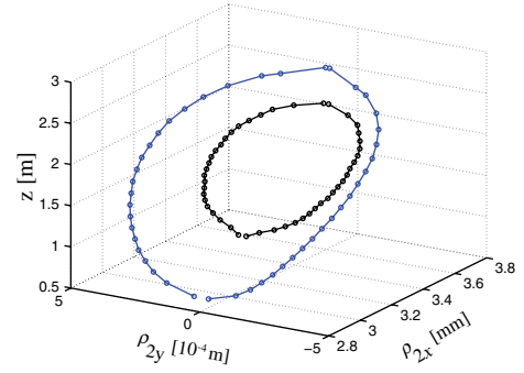
Fig. 6. (Color online) Two strings of correlation singularities in a partially coherent beam. The larger string (blue) is for \delta_{yy} = 0.09 mm, and the shorter string (black) is for the case \delta_{yy} = 0.12 mm.
