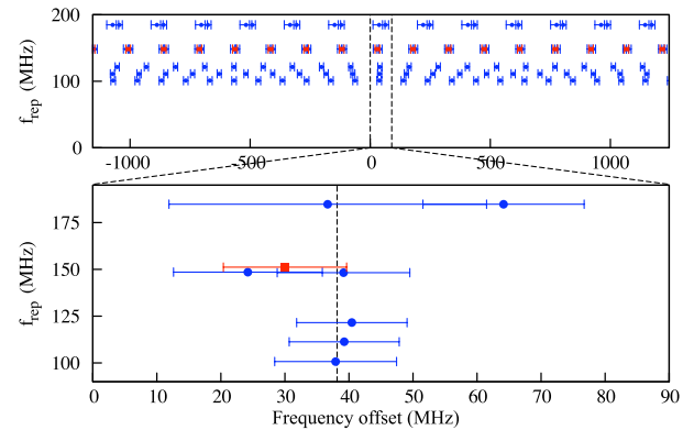
FIG. 3 (color online). (top) ^4\text{He} ground state ionization energy \pm n \times f_{\text{rep}} based on the 1s^2\ ^1S_0 - 1s5p\ ^1P_1 (blue circles) and the 1s^2\ ^1S_0 - 1s4p\ ^1P_1 transition (red squares). (bottom) Zoom at the coincidence point for all repetition frequencies. The vertical line at +38(6) MHz represents the weighted mean. All values are relative to the theoretical value of 5945 204 174 MHz [26]. (square point slightly shifted up for visibility).
