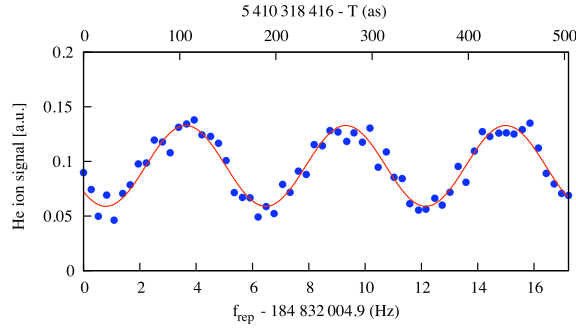
FIG. 2 (color online). Measured excitation probability (blue circles) of helium at 51.5 nm on the 1s^2\ ^1S_0 - 1s5p\ ^1P_1 transition, normalized by the XUV pulse energy, as a function of the repetition rate f_{\text{rep}} of the frequency-comb laser. In this example f_{\text{CEO}} is locked at 46.21 MHz, and a 1:5 He:Ne mixture is used for the atomic beam. The red line is a fit to the data.
