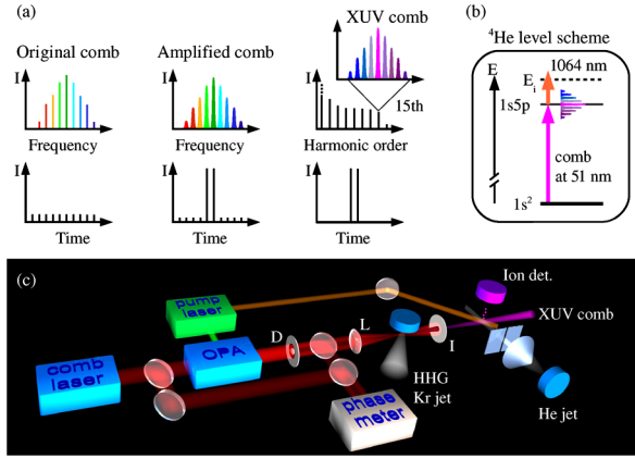
FIG. 1 (color online). (a) Spectral and temporal structure of the generated light (left to right): FC of the continuous coherent pulse train from the FC laser, the cosine-modulated spectrum of a pair of amplified pulses, and odd harmonics of the amplified FC laser pulses each containing a cosine-modulated XUV comb corresponding to the XUV pulse pair. (b) Simplified ^4\text{He} level scheme, XUV comb excitation at 51.5 nm from the 1s^2 ground state to the 1s5p excited state and state-selective ionization by a pulse at 1064 nm. (c) Schematic of the experimental setup. D : beam mask, L : focusing lens, f = 50 cm, I : iris to separate XUV from IR. The pump laser provides both the 532 nm for pumping the OPA as well as 1064 nm for ionization of helium.
