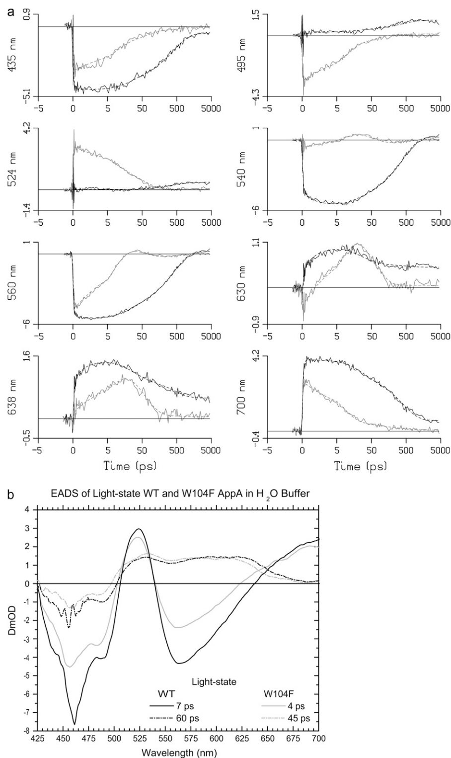
FIGURE 3 (a) Kinetic traces recorded in the AppA BLUF domain in H 2 O buffer on excitation at 400 nm in the dark state (black lines) and the light state (gray lines). Conversion to the light state was carried out through background illumination. The solid lines denote experimental data; the gray solid lines contain an estimated fraction of 10% of the dark-state photocycle; and the dashed lines are fits from a global analysis. Note that the time axis is linear up to 5 ps and logarithmic thereafter. (b) EADS that follow from a global analysis of the light-state (background-illuminated) time-resolved data of wild-type (black lines) and W104F mutant (gray lines) AppA BLUF in H 2 O buffer.
