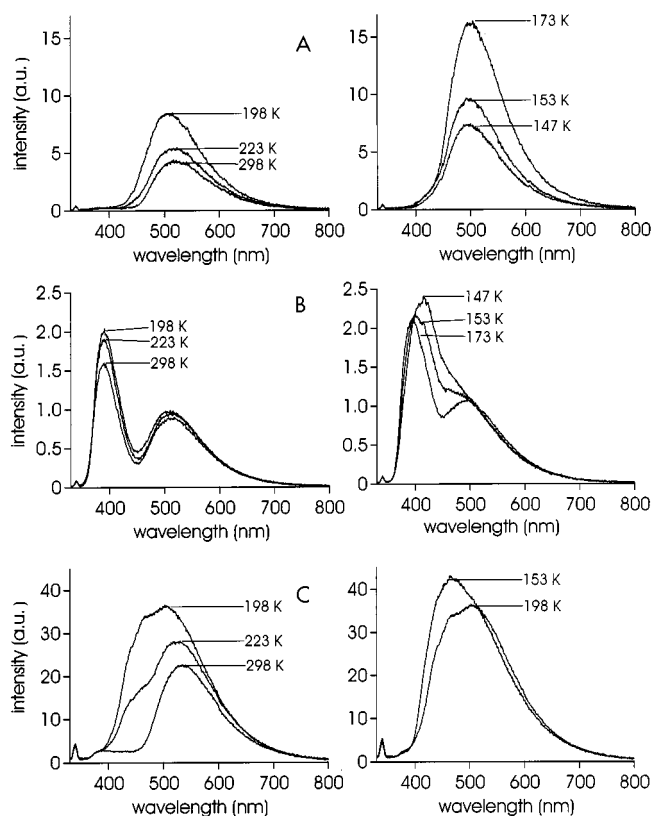
Figure 9. Fluorescence spectra of 5b (A), 6b (B), and 7b (C) in methylcyclohexane at different temperatures, excitation wavelength 308 nm
