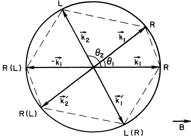
FIG. 4. Typical paths contributing to the two helicity channels. The helicities of the reversed path are labeled both for the Helicity-preserving channel as well as for the opposite helicity channel (in parentheses).
