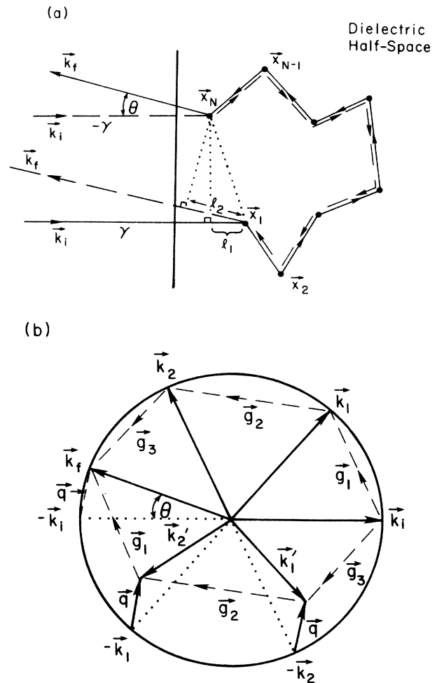
FIG. 1. (a) A typical scattering path ( \gamma ) in real space and the time reverse ( -\gamma ) with which it coherently interferes for small \theta . The phase difference between \gamma and -\gamma is simply proportional to the path length difference l_2 - l_1 , where l_1 = (\mathbf{x}_1 - \mathbf{x}_N) \cdot \hat{\mathbf{k}}_i and l_2 = (\mathbf{x}_N - \mathbf{x}_1) \cdot \hat{\mathbf{k}}_f . (b) A typical path drawn in momentum space. Equality of the scattering amplitudes requires that the wave-vector transfers \mathbf{g}_j be the same but in the reverse order for the time-reversed path. Corresponding states differ in energy by an amount E_{N-j} - E'_j \simeq c\hbar\mathbf{q} \cdot \hat{\mathbf{k}}_j , which leads to a phase difference (\Delta\phi)_{\text{rms}} \simeq \sqrt{N/3}ql .
