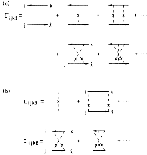
FIG. 5. The correlation \Gamma_{ijkl} = \langle G_{ik}^R G_{lj}^A \rangle can be evaluated by the sum of diagrams in (a). The solid lines denote the Green's functions G^{R/A} with the labeled indices and the dashed lines represent scattering. In the white-noise approximation of the disorder, these dashed lines carry a constant factor ( \gamma ) in momentum space. The principal contributions for k_0 l \gg 1 to \Gamma involve the ladder L and maximally crossed diagrams C , which may be evaluated by the sums in (b). The first term in the sum for L corresponds to single scattering and does not contribute to the helicity-preserving intensity.
