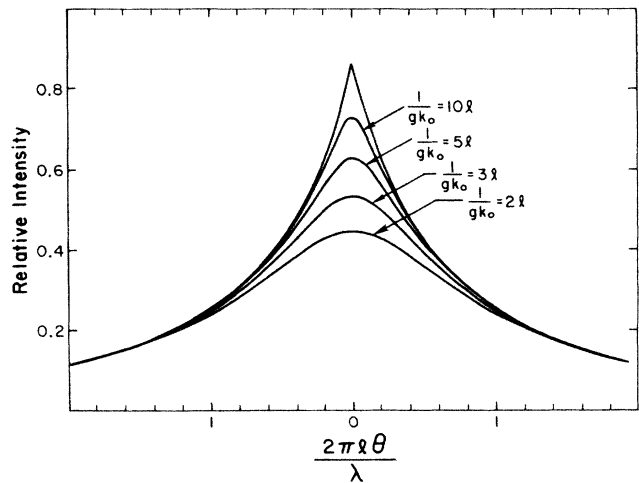
FIG. 6. The effect of Faraday rotation on the peak intensity of light polarized parallel to the incident wave. In the presence of time-reversal symmetry, the enhancement factor at \theta=0 is somewhat less than 1.9—we have normalized by the isotropic background in this channel. Also, the suppression of the peak due to time-reversal symmetry breaking is less severe than in the helicity-preserving channel or for scalar waves.
