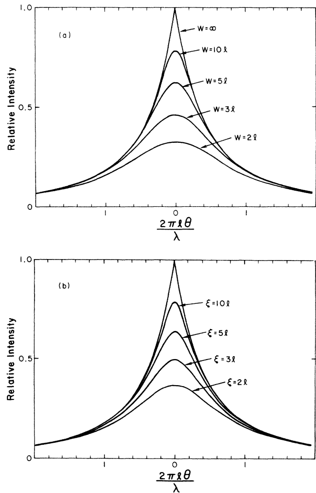
FIG. 2. The calculated scalar coherent backscattering line shapes. (a) As the width W of the scattering medium is reduced the central portion of the peak is suppressed by the termination of scattering paths. (b) Similarly the peak is reduced as absorption (with length l_i ) is introduced. These curves are labeled by the mean penetration depth \xi = (l_i/3)^{1/2} , which decreases with stronger absorption. Curves (a) and (b) are quite similar, with the correspondence W \leftrightarrow \xi . These curves represent the coherent peak, from which the isotropic background has been subtracted. The curves have then been normalized by the isotropic background intensity. Thus, the coherent peak of unit relative intensity corresponds to an actual enhancement factor of 2 in the total reflected intensity.
