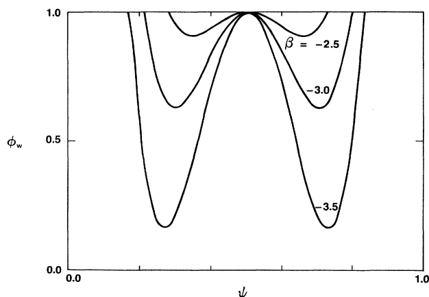
FIG. 2. Stability boundary for the vesicle phase as a function of the composition asymmetry \psi and the water volume fraction \phi_w . Curves are shown for three values of the interaction parameter \beta . The figure is drawn for the case where the spontaneous curvatures of the two surfactants are positive (tending to make micelles in oil), c_1 = c_2 = 1/2\delta , where \delta is of order the surfactant size.
