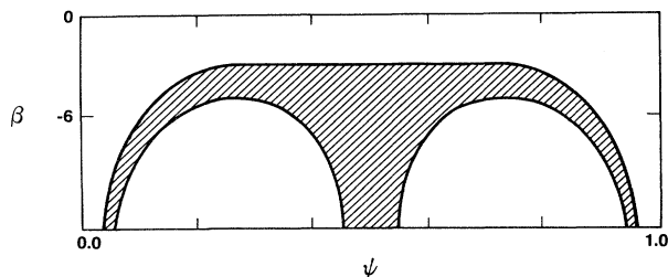
FIG. 1. Range of interaction strength where vesicles are stable (shaded area) as a function of the relative composition \psi . The figure is drawn for the case where the spontaneous curvatures of the two surfactants are positive (tending to make micelles in oil), c_1 = c_2 = 1/2\delta , where \delta is of order the surfactant size.
