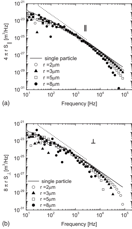
FIG. 8. Normalized displacement cross-correlation functions 4\pi r S_{||} (a) and 8\pi r S_{\perp} (b) of two probe particles (silica beads, R = 0.58 \mu\text{m} ) in worm-like micelle solutions ( c_m = 1 \text{ wt } \% ) versus frequency ( f = \omega/2\pi ) compared for different separation distances r . The solid lines represent the autocorrelation function of a single particle normalized by 6\pi R . The dashed lines indicate slopes of -2 , corresponding to diffusive motion.
