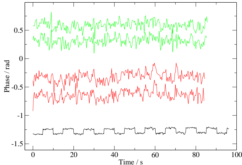
Fig. 6. Artificial phase shift measured with the interferometric switching technique (black/lower trace) and tested in a single interferogram for each pulse, with alternate switching the phase shift on and off (first pulse - green/upper traces, second pulse - red/middle traces).
