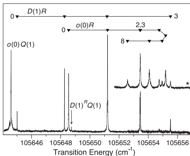
FIG. 3. 1 XUV+1 UV ionization spectrum of the R branches of the o^1\Pi_u-X^1\Sigma_g^+(0,0) and D^3\Sigma_u^+-X^1\Sigma_g^+(1,0) bands in ^{15}N_2 , recorded using the PDA-based XUV source. Nozzle-skimmer distance=150 mm, except for the scan labeled with an asterisk where the nozzle-skimmer distance = 0 mm.
