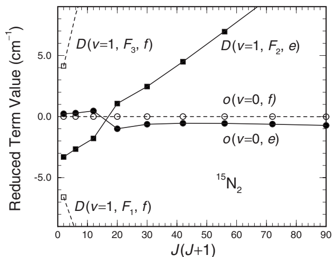
FIG. 4. Experimental reduced term values for e - and f -parity levels in the region of the o(v=0)\sim D(v=1) crossing in ^{15}N_2 (symbols). Terms have been reduced so that the o(v=0) f -parity levels lie on the zero line. The two D(v=1, f) level series, which are located above ( F_3 ) and below ( F_1 ) the D(v=1, e) level series, do not cross o(v=0) in the region covered by the figure. The fitted reduced terms resulting from the deperturbation procedure (see text) are also shown (solid lines: e levels and dashed lines: f levels).
