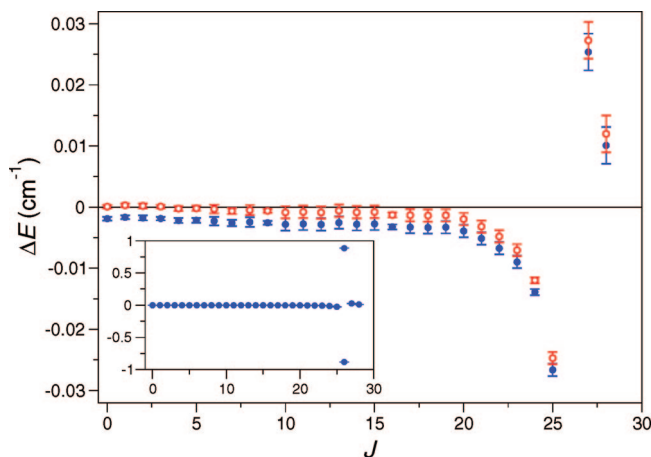
Figure 2. The perturbative shifts on the Q-branch transitions of a'' {}^1\Sigma_g^+ -X {}^1\Sigma_g^+(0,0) system. The filled circles (blue) represent the shifts in the case of a homogeneous perturbation while the unfilled circles (red) represent those in the case of heterogeneous perturbation. The inset shows an overview to include the J = 26 transitions, with the upper point representing the transition belonging to the perturber state.
