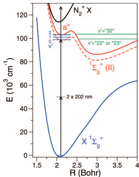
Figure 3. Potential energy curves for N_2 . In the adiabatic picture, a double-well potential is formed from the interaction of the a''^1\Sigma_g^+ and 1\Sigma_g^+(II) states. While the solid curve for the a''^1\Sigma_g^+(II) represents the data from Ermler et al., 19 the dashed curve is the potential that was shifted down by Bominaar et al., 20,26 to match the a''(0) level with observations. The horizontal lines indicate the experimentally observed energy levels.
