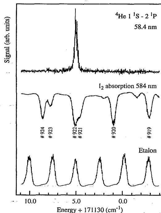
FIG. 2. The 1^1S \rightarrow 2^1P resonance line of ^4\text{He} at 58.4 nm recorded by 1 XUV+1 UV photoionization in the seeded beam. Also shown is part of an \text{I}_2 absorption spectrum in the visible as well as a Fabry-Pérot spectrum. We used the lines labeled 920 and 924 in the iodine atlas [14] for calibration.
