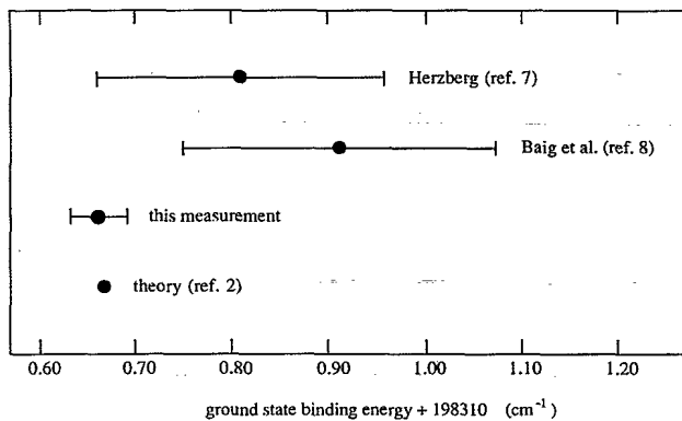
FIG. 3. Comparison of experimental and theoretical values for the binding energy of the {}^4\text{He } 1^1\text{S} ground state. The uncertainty for the theory is estimated to be on the order of 0.001 \text{ cm}^{-1} .
