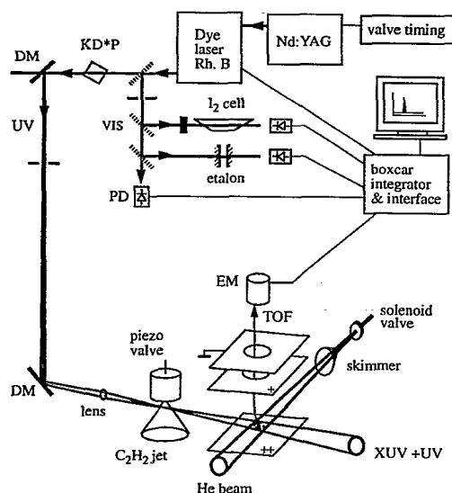
FIG. 1. Schematic of the experimental setup for XUV laser spectroscopy. DM: dichroic mirror; EM: electron multiplier; TOF: time of flight.
