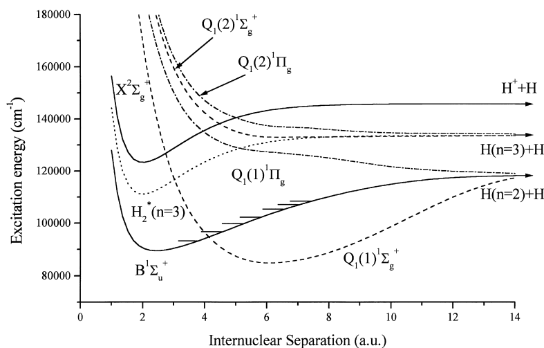
Fig. 1. Schematic potential energy diagram of molecular hydrogen, in which doubly excited repulsive Q_1 states [1] of ^1\Sigma_g^+ (dashed lines) or ^1\Pi_g symmetry (dashed-dots) and the bound H_2^*(n=3) Rydberg state (dotted lines) are shown. A quasidiabatic representation is presented, ignoring the interactions between the Rydberg states and the doubly excited states. The v' = 3, 5, 8, 11, 14, 17 and 20 are indicated in the B state.
