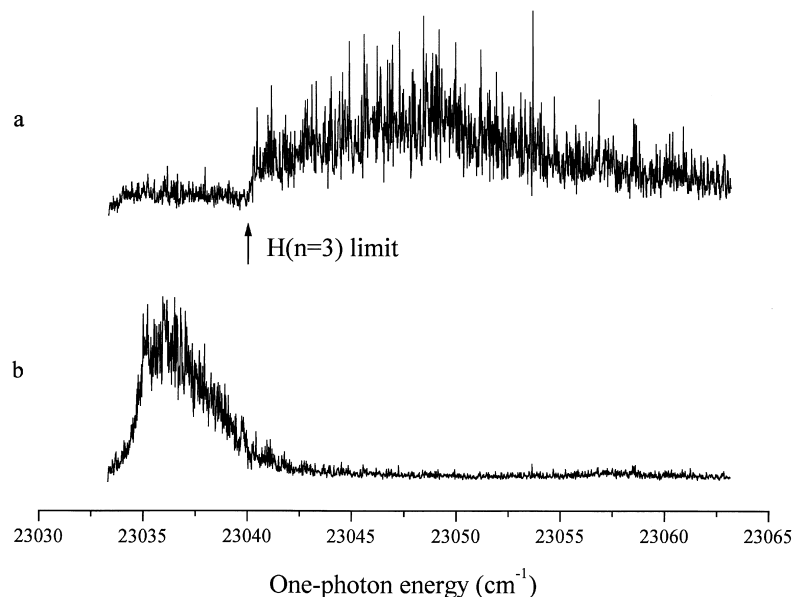
Fig. 3. Two-colour excitation spectra obtained by fixing one laser on the B^1\Sigma_u^+(v'=20, J'=2) \leftarrow X^1\Sigma_g^+(v''=0, J''=1) transition, while the second laser is scanned across the H(n=1) + H(n=3) dissociation limit. The frequency of the second laser is given along the horizontal axis. In (a) and (b) the H^+ signal from ionization of n=3 fragments and the H_2^+ signal are shown, respectively.
