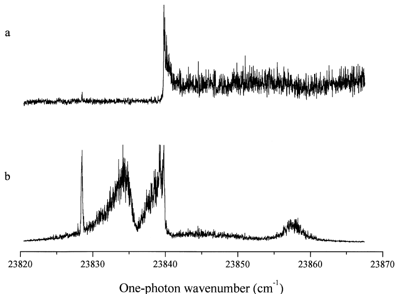
Fig. 4. Two-colour excitation spectra obtained by fixing one laser on the \text{B}^1\Sigma_u^+(v' = 19, J' = 0) \leftarrow \text{X}^1\Sigma_g^+(v'' = 0, J'' = 1) transition, while the second laser is scanned across the \text{H}(n = 1) + \text{H}(n = 3) dissociation limit. The frequency of the second laser is given along the horizontal axis. In (a) and (b) the \text{H}^+ signal from ionization of n = 3 fragments and the \text{H}_2^+ signal are shown, respectively. This example clearly shows the closing of the autoionization channel on a broad resonance of \text{H}_2 at the \text{H}(n = 3) limit.
