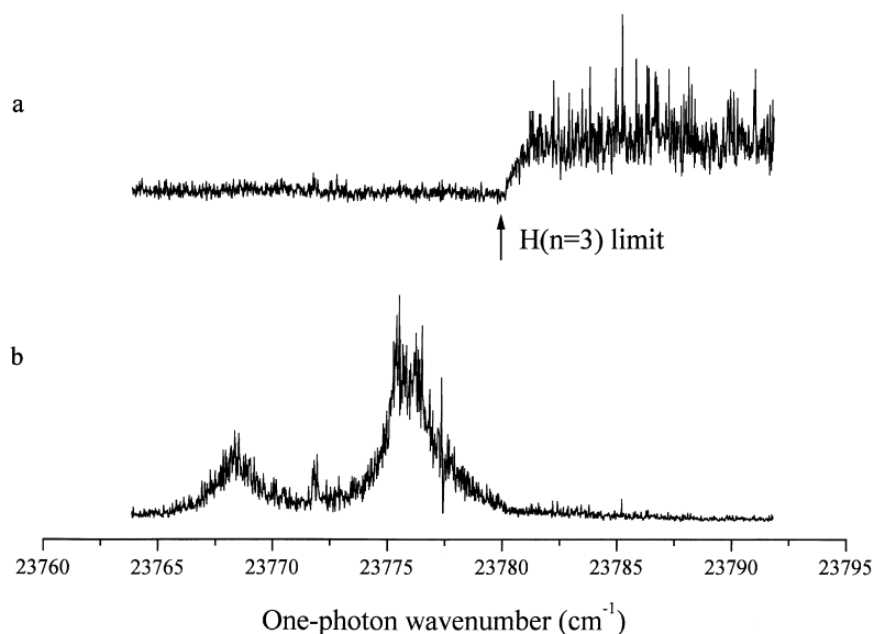
Fig. 2. Two-colour excitation spectra obtained by fixing one laser on the B^1\Sigma_u^+(v'=19, J'=2) \leftarrow X^1\Sigma_g^+(v''=0, J''=1) transition, while the second laser is scanned across the H(n=1) + H(n=3) dissociation limit. The frequency of the second laser is given along the horizontal axis. In (a) and (b) the H^+ signal from ionization of n=3 fragments and the H_2^+ signal are shown, respectively.
