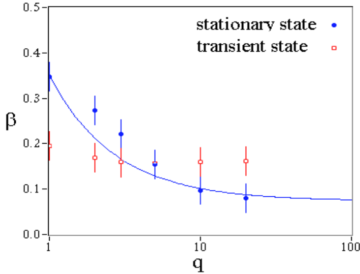
Fig. 4 – The dependence of the growth exponent \beta on the moment of the correlation function q , for both the stationary and the transient state, determined in the region of 1-60 and 1-30 time steps respectively. With increasing moment, \beta decreases in the stationary state, indicating multi-scaling. The solid line indicates the expectation for a SOC system in the stationary state (eq. 4), which is in reasonable agreement with the experimental results. In the transient state however, \beta does not depend on the moment of the correlation function q , indicating generic scaling. Again this is expected for a SOC system due to the absence of the critical correlation length in the transient state.
