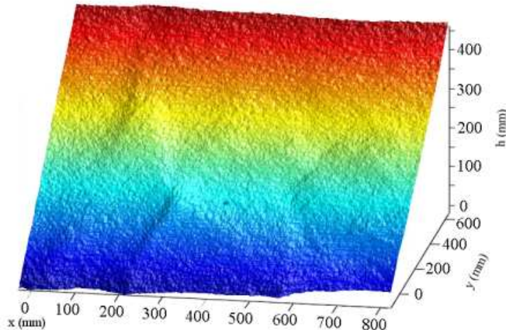
Fig. 1 – Reconstruction of a typical rice pile surface. The surface coordinates are reconstructed using a technique based on the projection of a set of colored lines to identify lines of equal height. The resolution and accuracy of the reconstruction method are \sim 1 - 2 mm, comparable to the size of a grain of rice.
